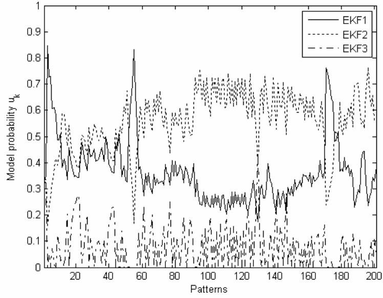
Figure 3.4. Model probabilities of each model for 1% noise.
