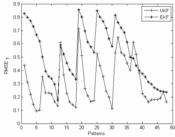
Figure 5.21. RMSE comparison for the second experiment.
