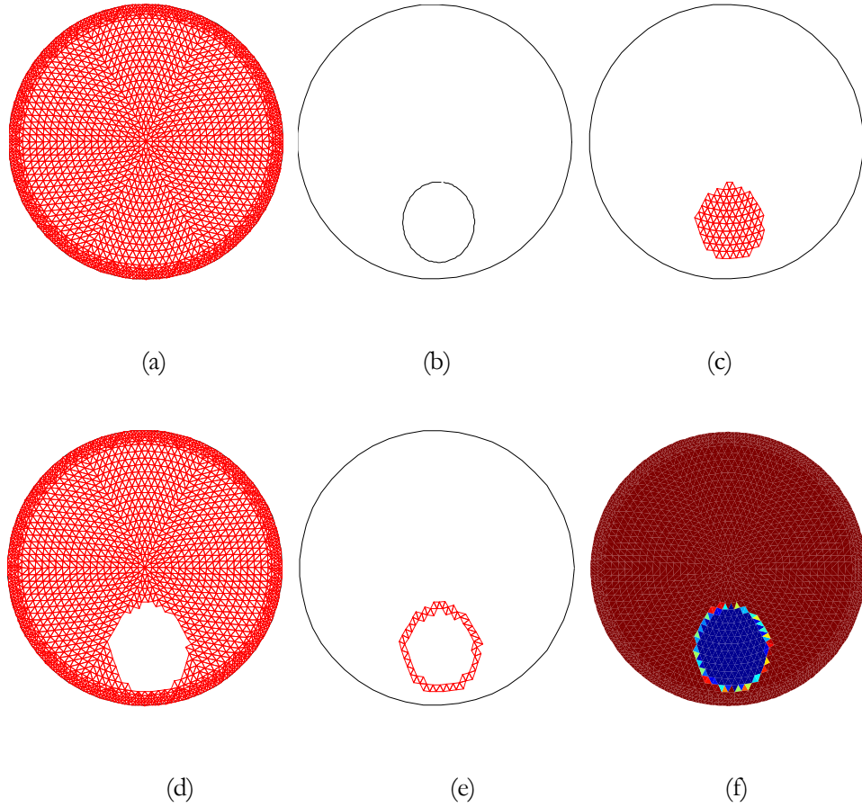
Figure 1.9. Fourier coefficients mapping to conductivity profile: (a) FEM discretization of the domain; (b) boundary represented by Fourier coefficients; (c) mesh elements belonging to target are assigned \sigma_I ; (d) mesh elements belonging to the background are assigned \sigma_r ; (e) mesh elements lying on the interface are assigned area average conductivity values assigned using equation (1.36); and (f) final conductivity values at the end of assignment.
