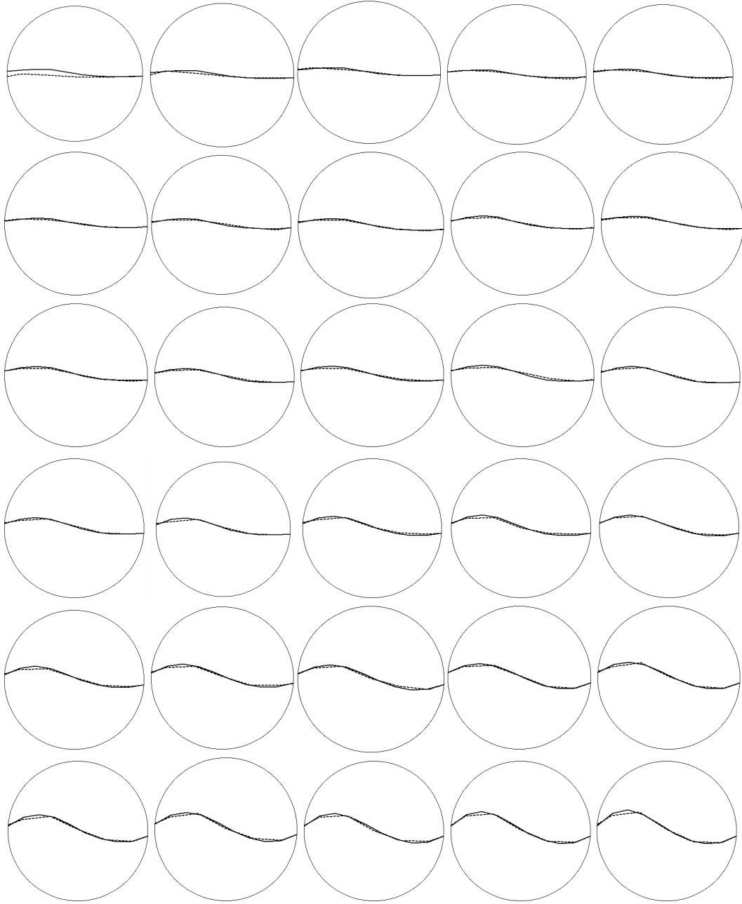
Figure 2.8. Reconstructed images for contrast ratio of 10:1 with 1% noise. The solid line represents the true interface and the dotted line represents the estimated interface.
