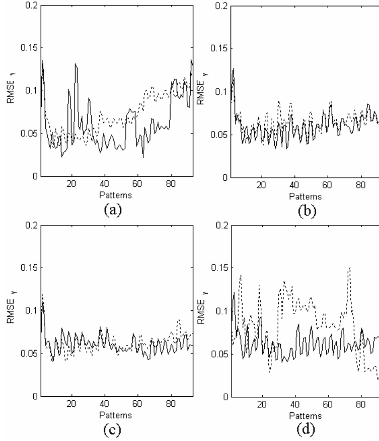
Figure 4.10. RMSE comparison with Monte-Carlo simulation of 10 runs: (a) bubble is moving with constant velocity; (b) bubble is expanding with constant velocity; (c) bubble is moving with constant velocity; and (d) bubble is expanding with constant acceleration. Solid line represents the RMSE with KM whereas dotted line represents the RMSE with random-walk model.
