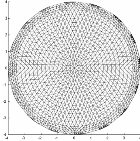
Figure 1.1. The FEM mesh with location of electrodes marked with darkened elements
