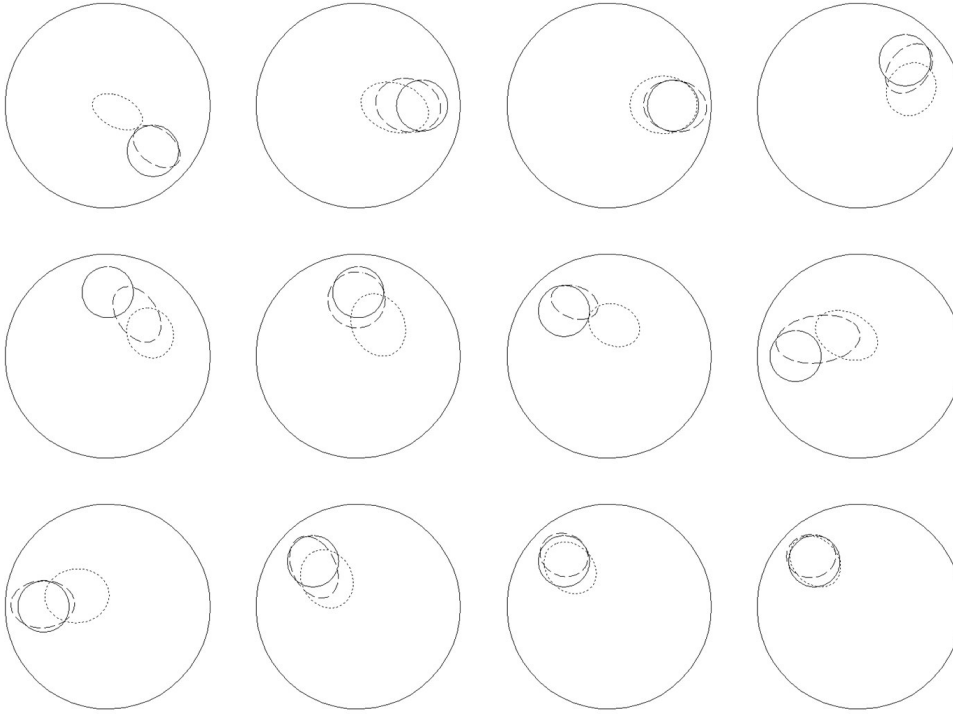
Figure 5.20. Reconstructed boundaries for the second experiment. Solid line, dotted line and dashed line represent the true boundary, boundary estimated by EKF, and boundary estimated by UKF, respectively.
