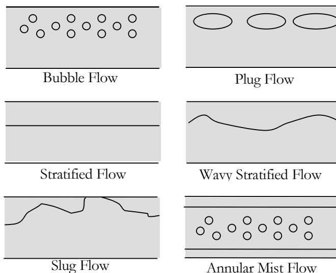
Figure 1. Different flow regimes observed with varying velocities in liquid-gas flow.
