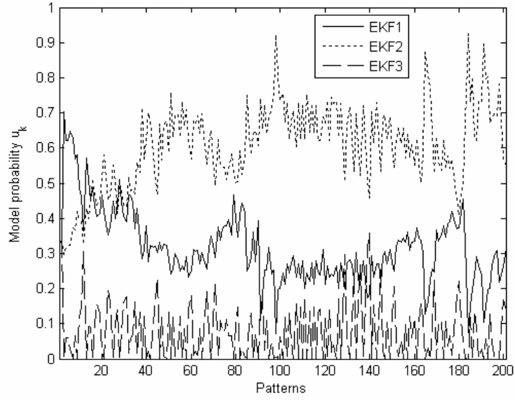
Figure 3.7. Model probabilities of each model for 2% noise.
