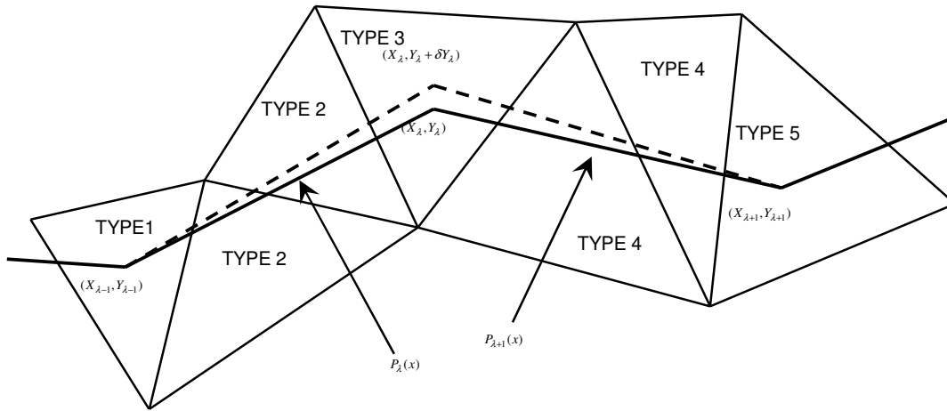
Figure 1.6. Five types of interface-crossing elements in case of an arbitrarily small perturbation of \delta Y_\lambda in Y_\lambda .
