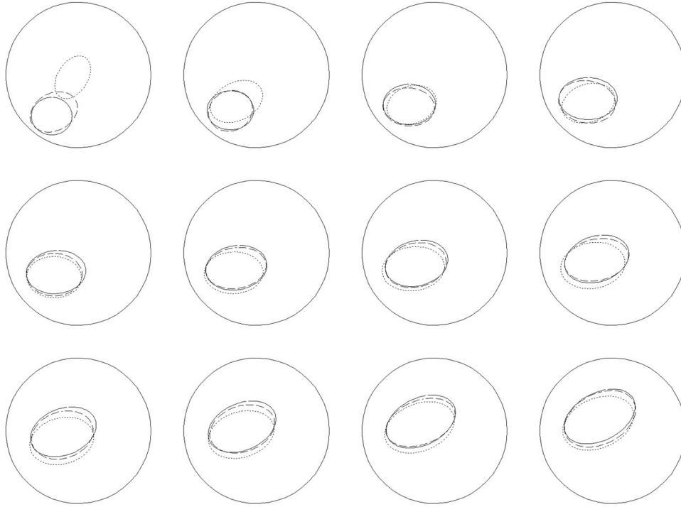
Figure 5.14. Reconstructed boundaries for scenario 2 with 2% noise. Solid line, dotted line and dashed line represent the true boundary, boundary estimated by EKF, and boundary estimated by UKF, respectively.
