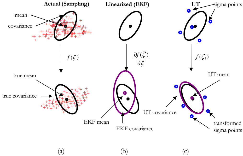
Figure 5.1. An example of unscented transform for mean and covariance propagation: (a) actual; (b) first-order linearization (EKF); and (c) unscented transform.
