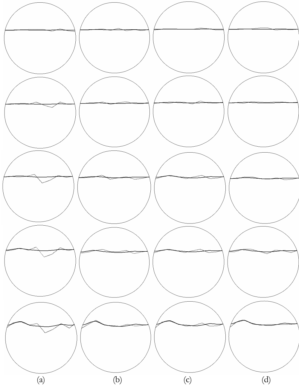
Figure 3.6. The reconstructed phase boundaries for 2% noise. The true boundaries are solid lines and the reconstructed boundaries are dotted lines: (a) boundaries reconstructed by the EKF1; (b) boundaries reconstructed by the EKF2; (c) boundaries reconstructed by the EKF3; and (d) boundaries reconstructed by the IMM.
