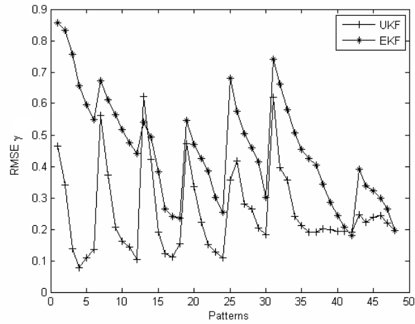
Figure 5.19. RMSE comparison for first experiment.
