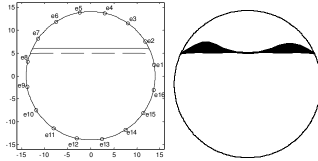
Figure 2.16. Description of the interfacial boundary movement where the interface is initially nearly flat and two ripples grow with time. The left profile describes the true (solid line) and the guessed (dotted line) initial boundary, respectively. Location of electrodes are also shown. The right profile shows the evolution of the interface.
