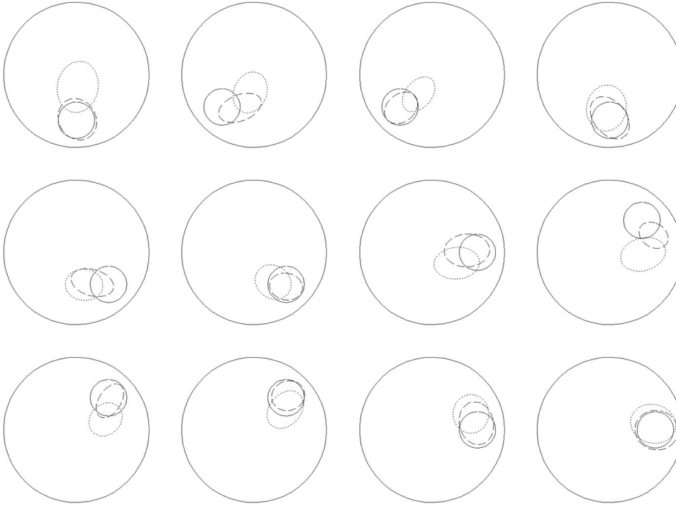
Figure 5.18. Reconstructed boundaries for first experiment. Solid line, dotted line and dashed line represent the true boundary, boundary estimated by EKF, and boundary estimated by UKF, respectively.
