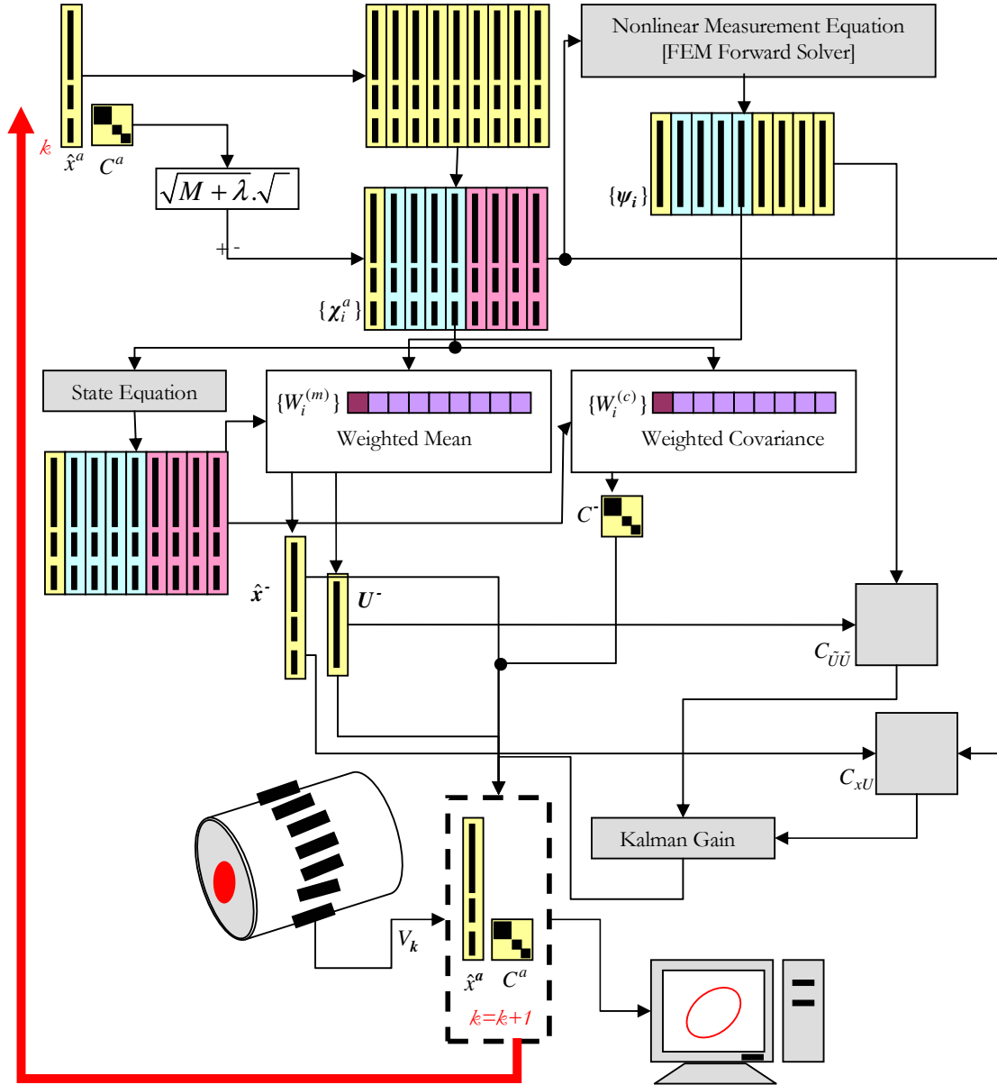
Figure 5.2. Block diagram of the UKF for phase boundary estimation in EIT.
