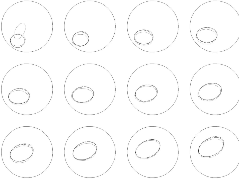
Figure 5.12. Reconstructed boundaries for scenario 2 with 1% noise. Solid line, dotted line and dashed line represent the true boundary, boundary estimated by EKF, and boundary estimated by UKF, respectively.
