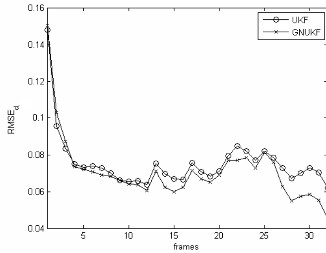
Figure 6.3. Results for 10 front points with 2% noise and contrast ratio of 100:1: (a) reconstructed boundaries after every 4 current patterns. True profile (—), GNUKF (—x—), and UKF (—o—); (b) RMSE comparison between GNUKF and UKF.
