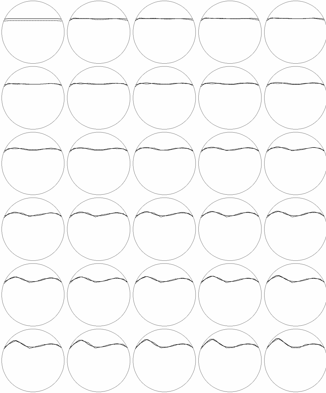
Figure 2.13. Reconstructed images for scenario 2 with 2% noise. The solid line represents the true interface and the dotted line represents the estimated interface.
