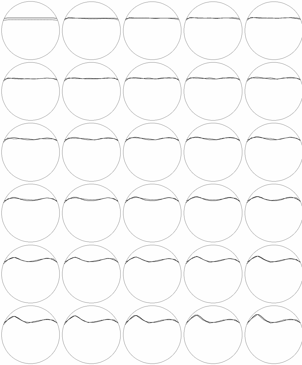
Figure 2.14. Reconstructed images for scenario 2 with 3% noise. The solid line represents the true interface and the dotted line represents the estimated interface.
