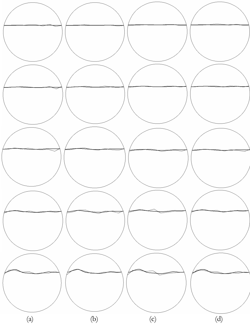
Figure 3.3. The reconstructed phase boundaries for 1% noise. The true boundaries are solid lines and the reconstructed boundaries are dotted lines: (a) boundaries reconstructed by the EKF1; (b) boundaries reconstructed by the EKF2; (c) boundaries reconstructed by the EKF3; and (d) boundaries reconstructed by the IMM.
