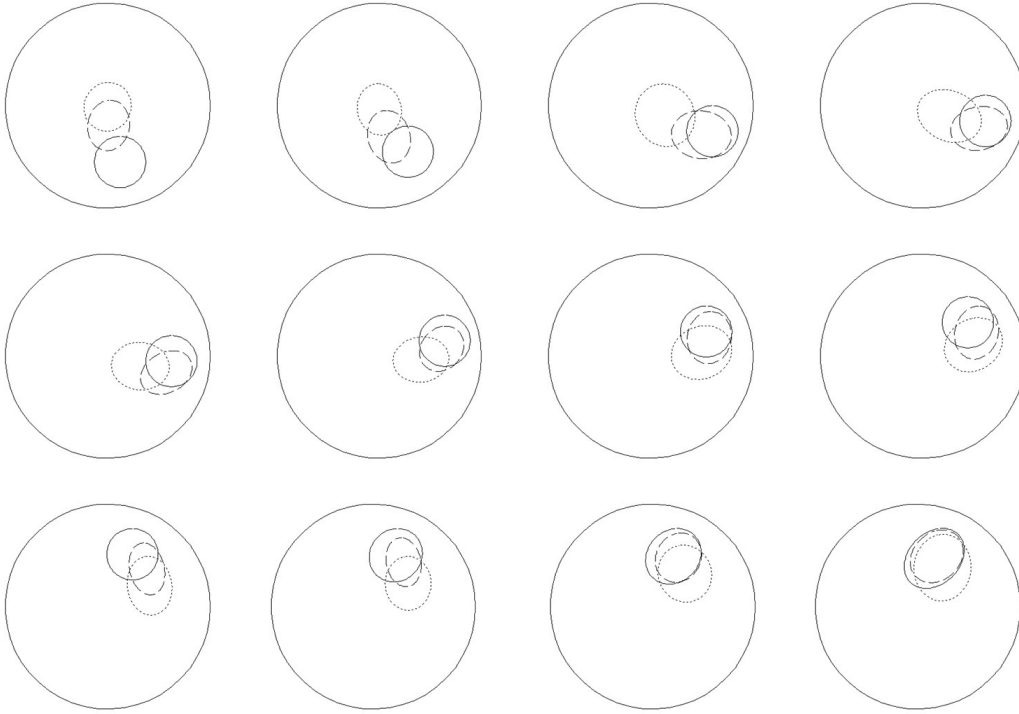
Figure 5.10. Reconstructed boundaries for scenario 1 with 3% noise. Solid line, dotted line and dashed line represent the true boundary, boundary estimated by EKF, and boundary estimated by UKF, respectively.
