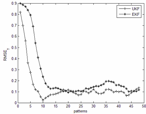
Figure 5.17. RMSE comparison for scenario 2 with 3% noise.
