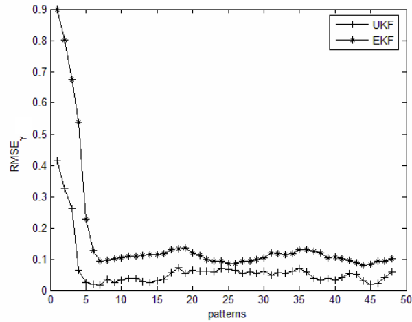
Figure 5.13. RMSE comparison for scenario 2 with 1% noise.
