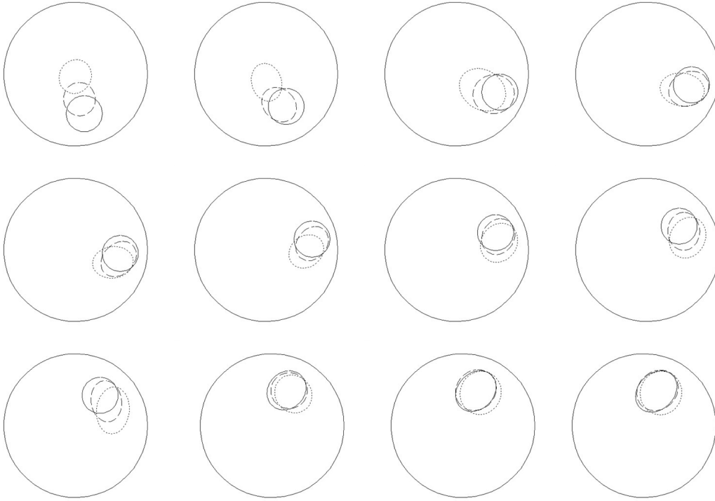
Figure 5.8. Reconstructed boundaries for scenario 1 with 2% noise. Solid line, dotted line and dashed line represent the true boundary, boundary estimated by EKF, and boundary estimated by UKF, respectively.
