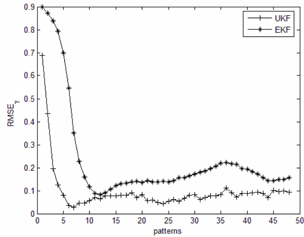
Figure 5.15. RMSE comparison for scenario 2 with 2% noise.
