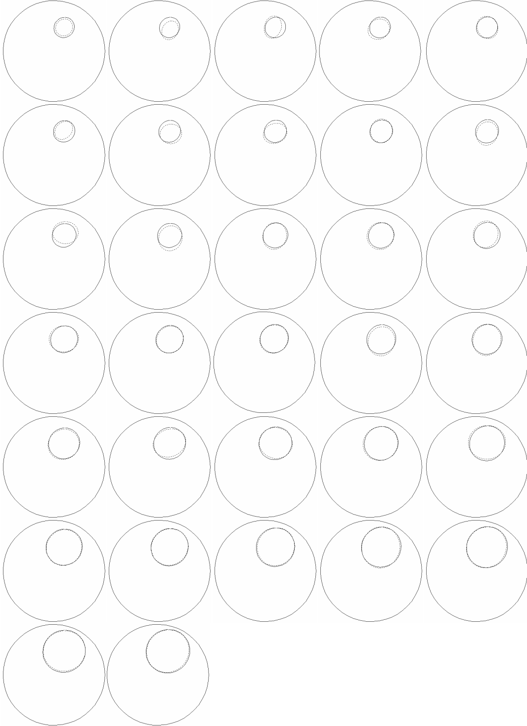
Figure 4.8. Reconstructed boundaries with kinematic model for bubble expanding with constant acceleration. True boundary is represented by solid line and estimated boundary is represented by dotted line.
