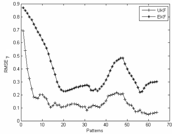
Figure 5.9. RMSE comparison for scenario 1 with 2% noise.
