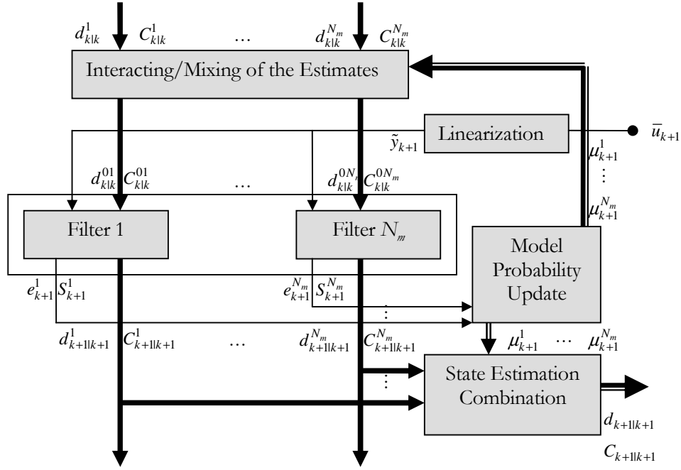
Figure 3.1. One-cycle flow diagram of the inverse solver with the IMM algorithm.
