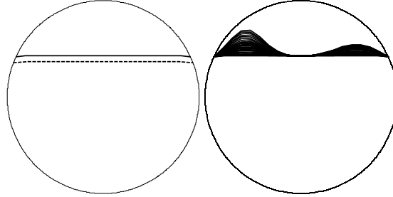
Figure 2.2. Description of the interfacial boundary movement in scenario 2 where the interface is initially nearly flat and two ripples grow with time. The left profile describes the true (solid line) and the guessed (dotted line) initial boundary, respectively. The right profile shows the evolution of the interface.
