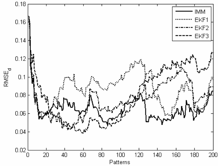
Figure 3.5. RMSE_d comparison between IMM and different EKFs for 1% noise.
