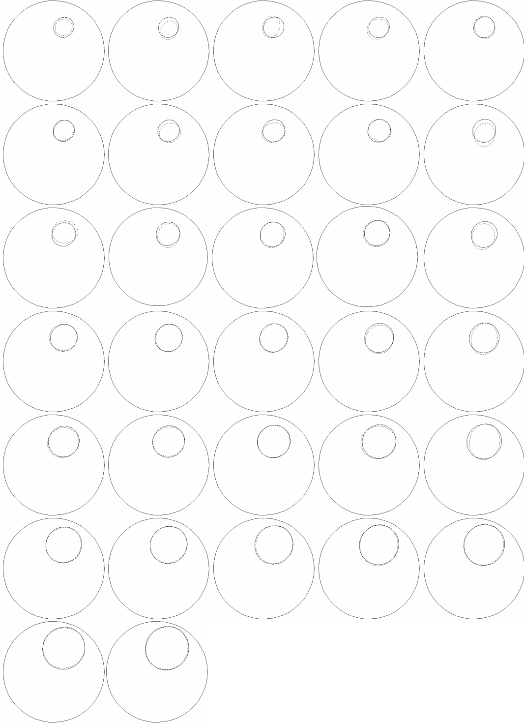
Figure 4.9. Reconstructed boundaries with random-walk model for bubble expanding with constant acceleration. True boundary is represented by solid line and estimated boundary is represented by dotted line.
