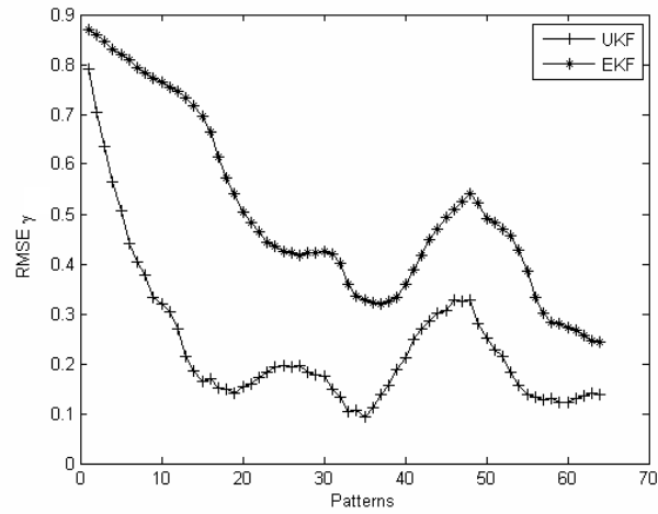
Figure 5.11. RMSE comparison for scenario 1 with 3% noise.
