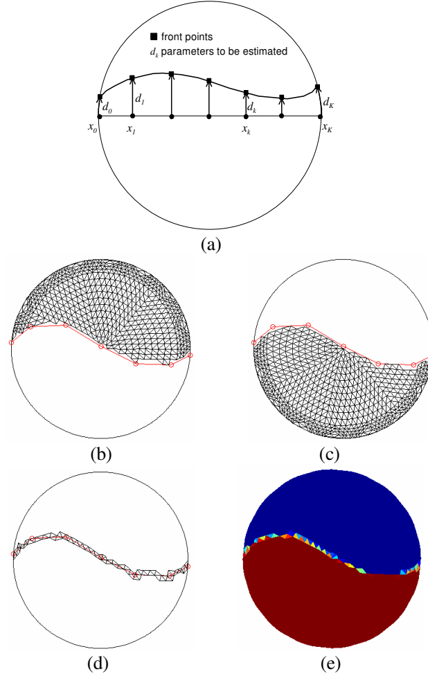
Figure 1.4. Problem representation: (a) description of interface with front points; (b) mesh elements above the interface are assigned \sigma_u ; (c) mesh elements below the interface are assigned \sigma_l ; (d) mesh elements lying on the interface are assigned area average conductivity values assigned using equation (1.36); and (e) final conductivity values at the end of assignment.
