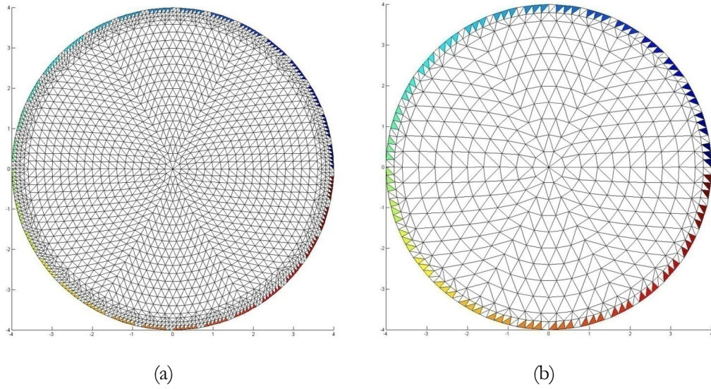
Figure 5.4. Meshes used in: (a) forward solver; and (b) inverse solver.
