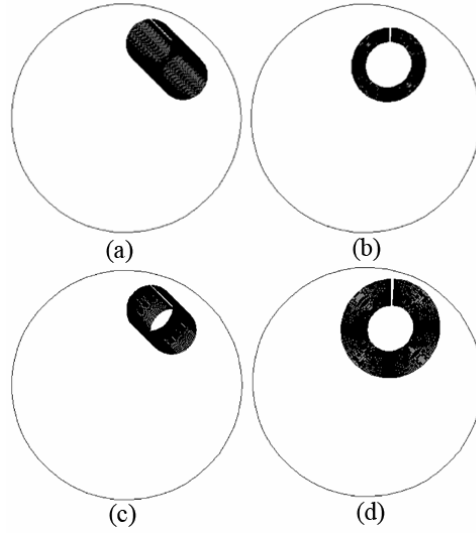
Figure 4.1. Scenarios for kinematic model: (a) bubble is moving with constant velocity; (b) bubble is expanding with constant velocity; (c) bubble is moving with constant acceleration; and (d) bubble is expanding with constant acceleration. Transient boundaries are superimposed onto each other.
