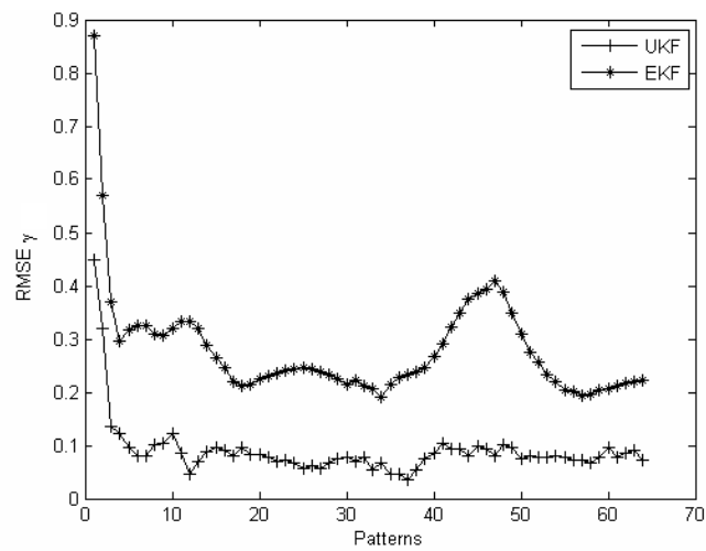
Figure 5.7. RMSE comparison for scenario 1 with measurements perturbed by 1% white Gaussian noise.
