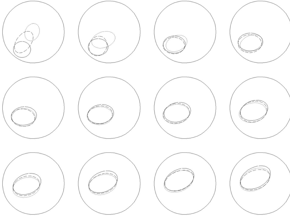
Figure 5.16. Reconstructed boundaries for scenario 2 with 3% noise. Solid line, dotted line and dashed line represent the true boundary, boundary estimated by EKF, and boundary estimated by UKF, respectively.
