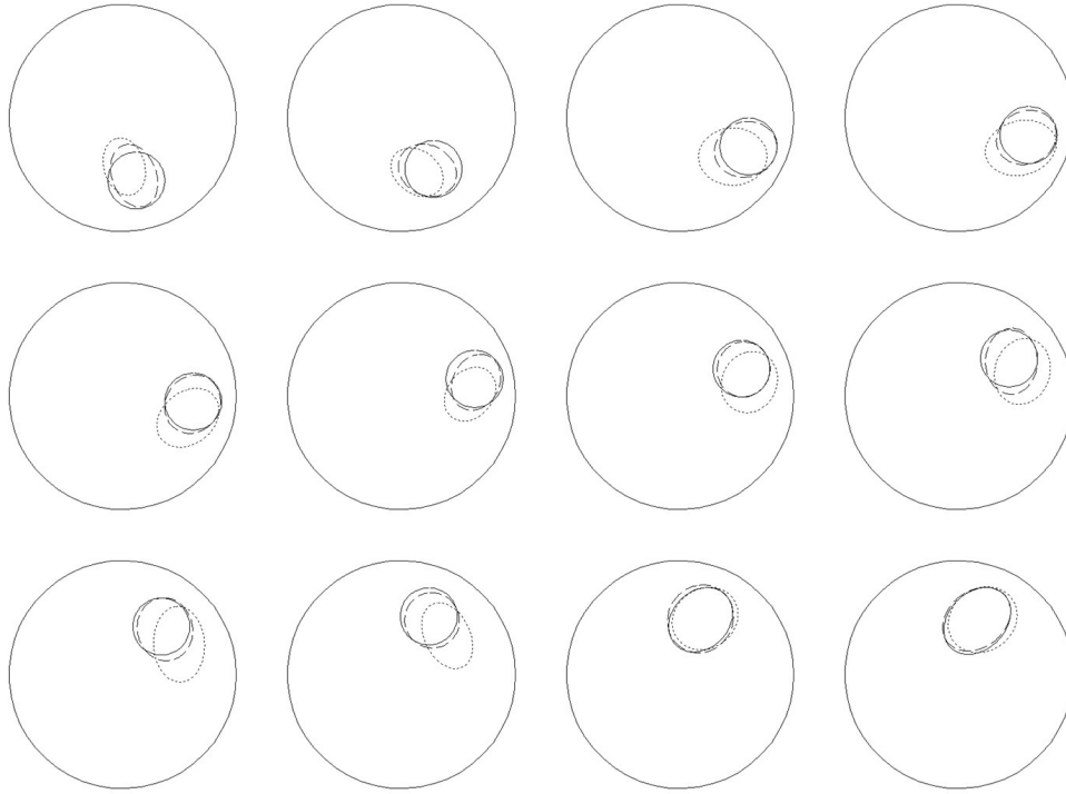
Figure 5.6. Reconstructed boundaries for scenario 1 with 1% noise. Solid line, dotted line and dashed line represent the true boundary, boundary estimated by EKF, and boundary estimated by UKF, respectively.
