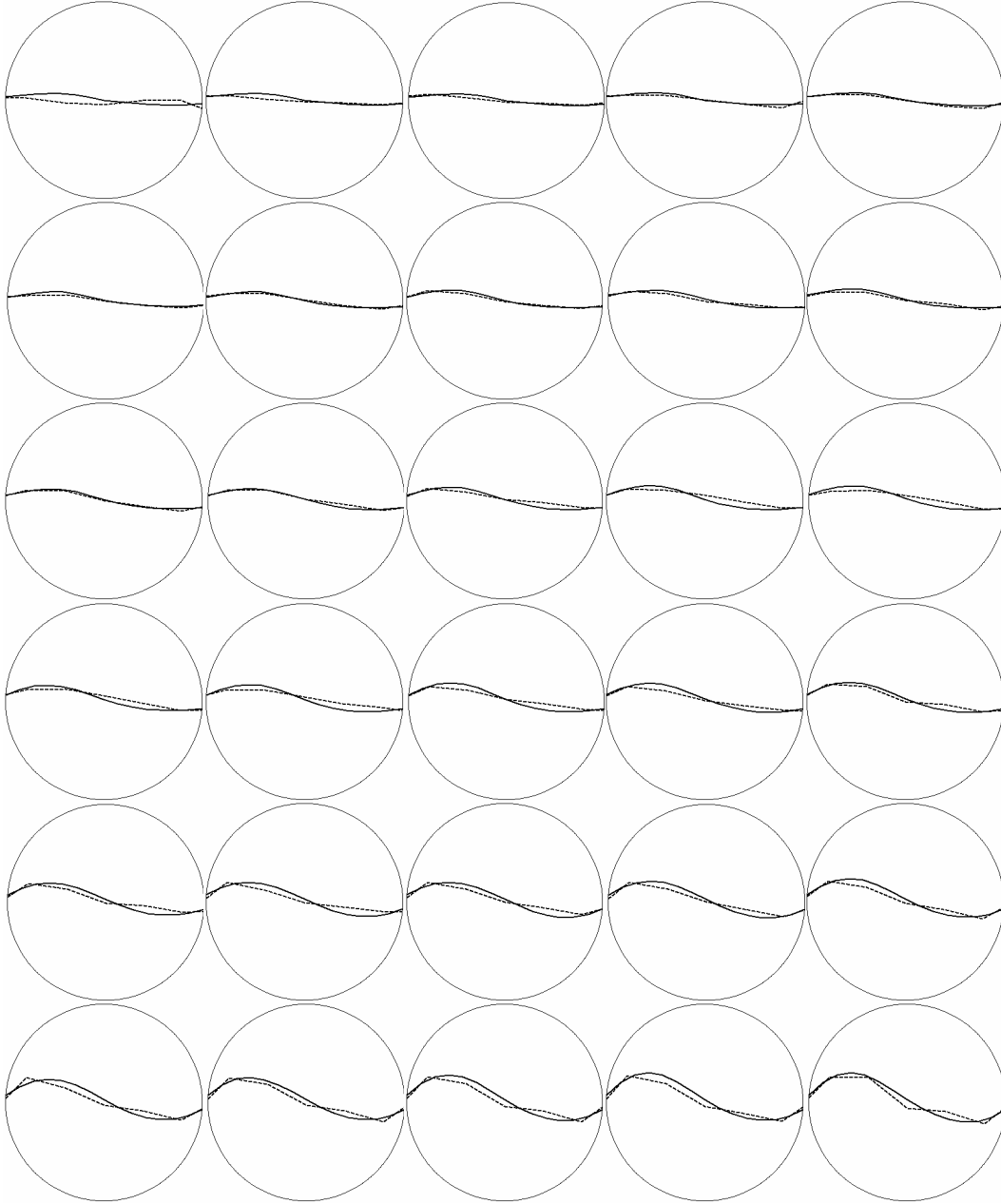
Figure 2.5. Reconstructed images for scenario 1 with 3% noise. The solid line represents the true interface and the dotted line represents the estimated interface.
