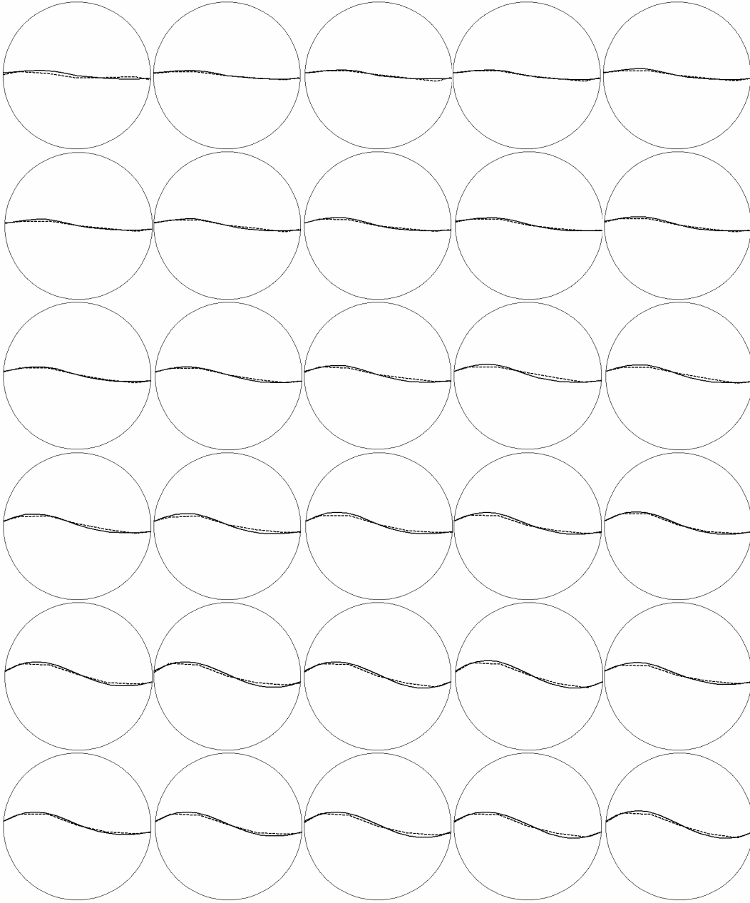
Figure 2.3. Reconstructed images for scenario 1 with 1% noise. The solid line represents the true interface and the dotted line represents the estimated interface.
