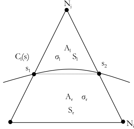
Figure 1.3. A schematic representation of FEM element \Omega_e intercepted by the phase boundary C_l(s) .
