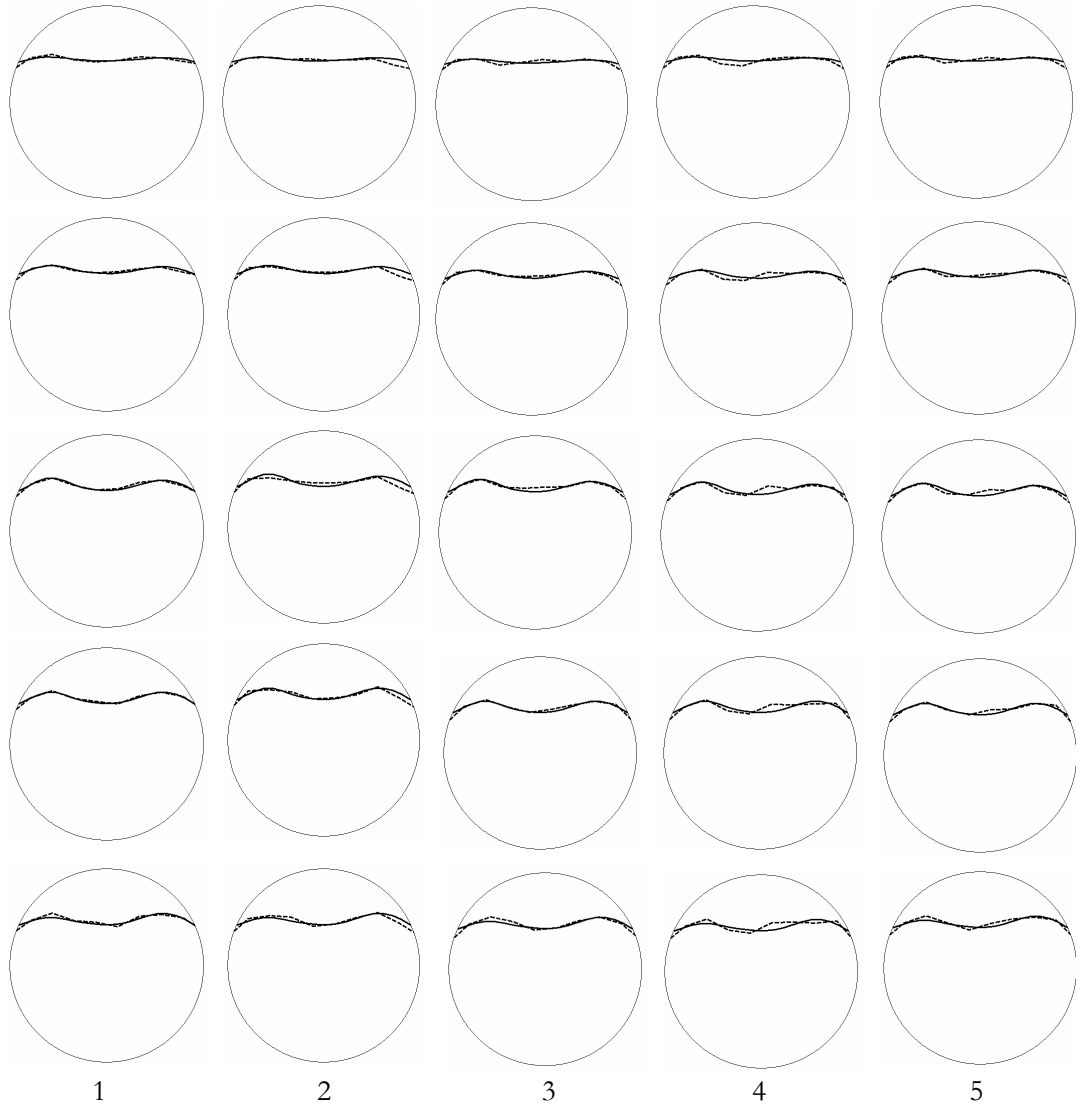
Figure 2.17. Reconstructed images for scenario 3 with 1% noise. The solid line represents the true interface and the dotted line represents the estimated interface.
