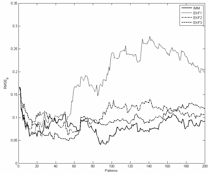
Figure 3.8. RMSE_d comparison between IMM and different EKF's for 2% noise.
