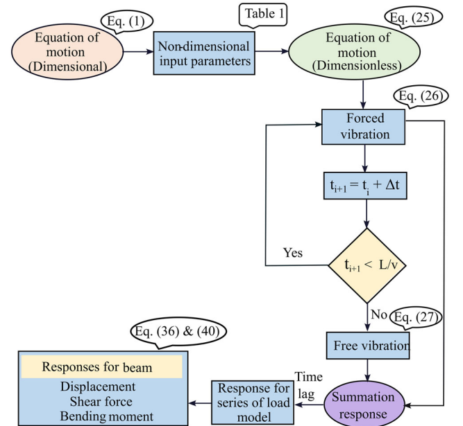
Figure 3. Flowchart of the proposed analytical model.
