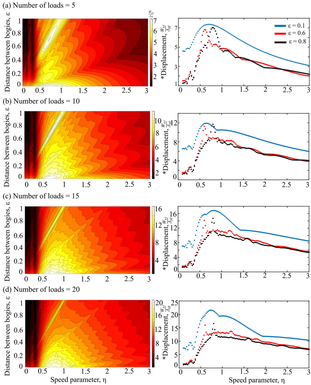
Figure 11. *Dimensionless displacement response for (a) number of loads = 5; (b) number of loads = 10; (c) number of loads = 15; and (d) number of loads = 20 for HSLM-B.
