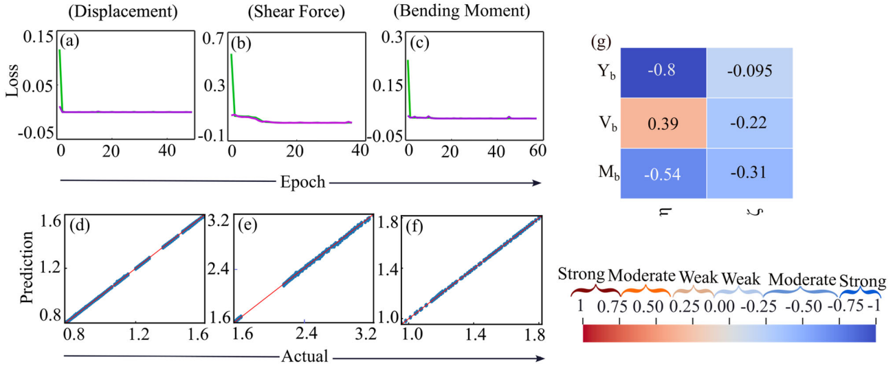
Figure 9. Loss versus epoch for (a) displacement; (b) shear force; (c) Bending moment; Prediction versus actual for (d) displacement; (e) shear force; (f) bending moment; and (g) Pearson correlation matrix with speed parameter \eta and damping \zeta for single load model.
