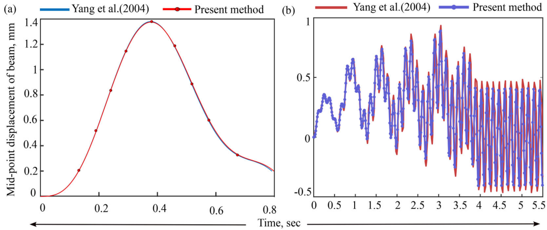
Figure 6. Comparison of the mid-point displacement response of the simply-supported beam for (a) single moving load; (b) Series of load as per HSLM-B model.
