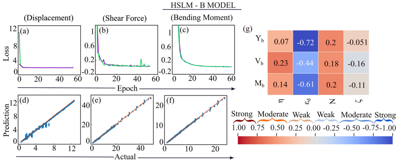
Figure 13. Loss versus epoch for (a) displacement; (b) shear force; (c) bending moment; Prediction versus actual for (d) displacement; (e) shear force; (f) bending moment; and (g) Pearson correlation matrix for HSLM-B with speed parameter \eta , distance between loads to the length of the bridge \epsilon , number of loads N , and damping \zeta .
