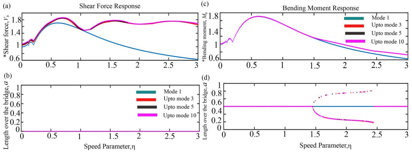
Figure 8. (a) *Dimensionless maximum shear force \frac{V_b}{\Delta_{st}} versus speed parameter \eta ; (b) position of maximum amplitude of \frac{V_b}{\Delta_{st}} over the length of the bridge a versus speed parameter \eta ; (c) *Dimensionless maximum bending moment \frac{M_b}{\Delta_{st}} versus speed parameter \eta ; (d) Position of maximum amplitude of \frac{M_b}{\Delta_{st}} over the length of the bridge a versus speed parameter \eta .
