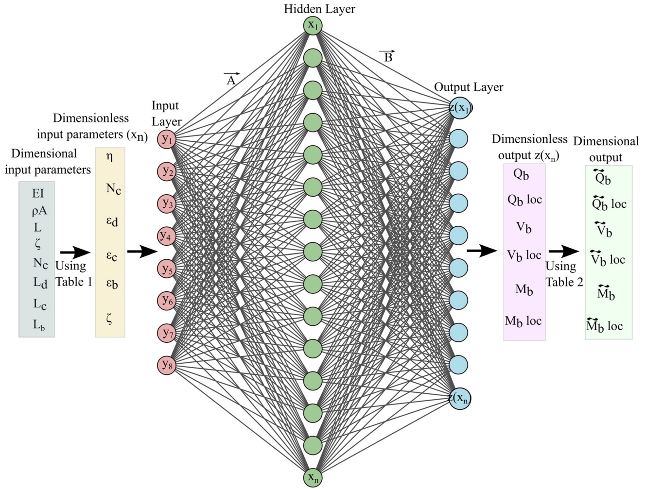
Figure 4. Architecture of ANN network diagram for MIMO model.
