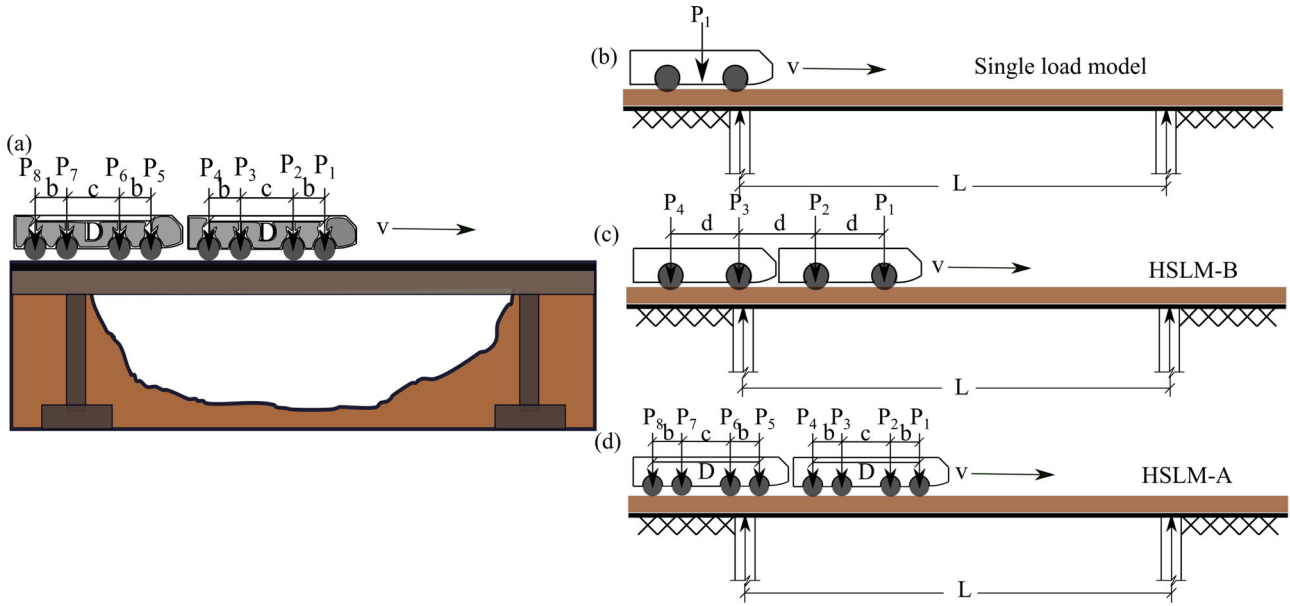
Figure 1. (a) Conceptualisation of model of elevated simply-supported bridge unit under the action of moving loads; (b) simplified idealisation of moving load as single load model; (c) simplified idealisation of series of moving load spaced at equidistant to each other (HSLM-B train model); and (d) simplified idealisation of series of loads as per conventional train model (HSLM-A train model).
