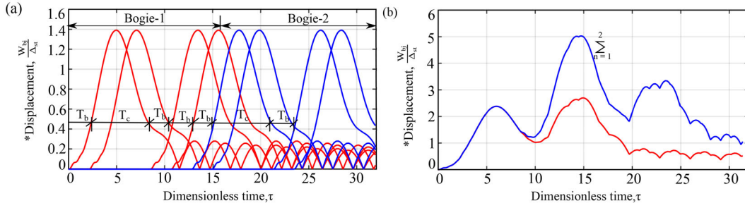
Figure 14. Conventional train model as bogie system with time lag, \epsilon_D = 0.1 , \epsilon_d = 0.1 for \eta = 0.4 as per HSLM-A (a)*Dimensionless displacement of 2 individual bogie; (b)*Dimensionless displacement of bogies in cumulative form.
