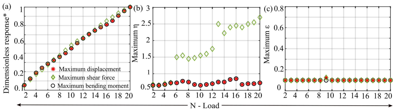
Figure 12. Variation of (a) *Normalised Dimensionless displacement response; (b) Maximum \eta ; (c) Maximum \epsilon for HSLM-B.
