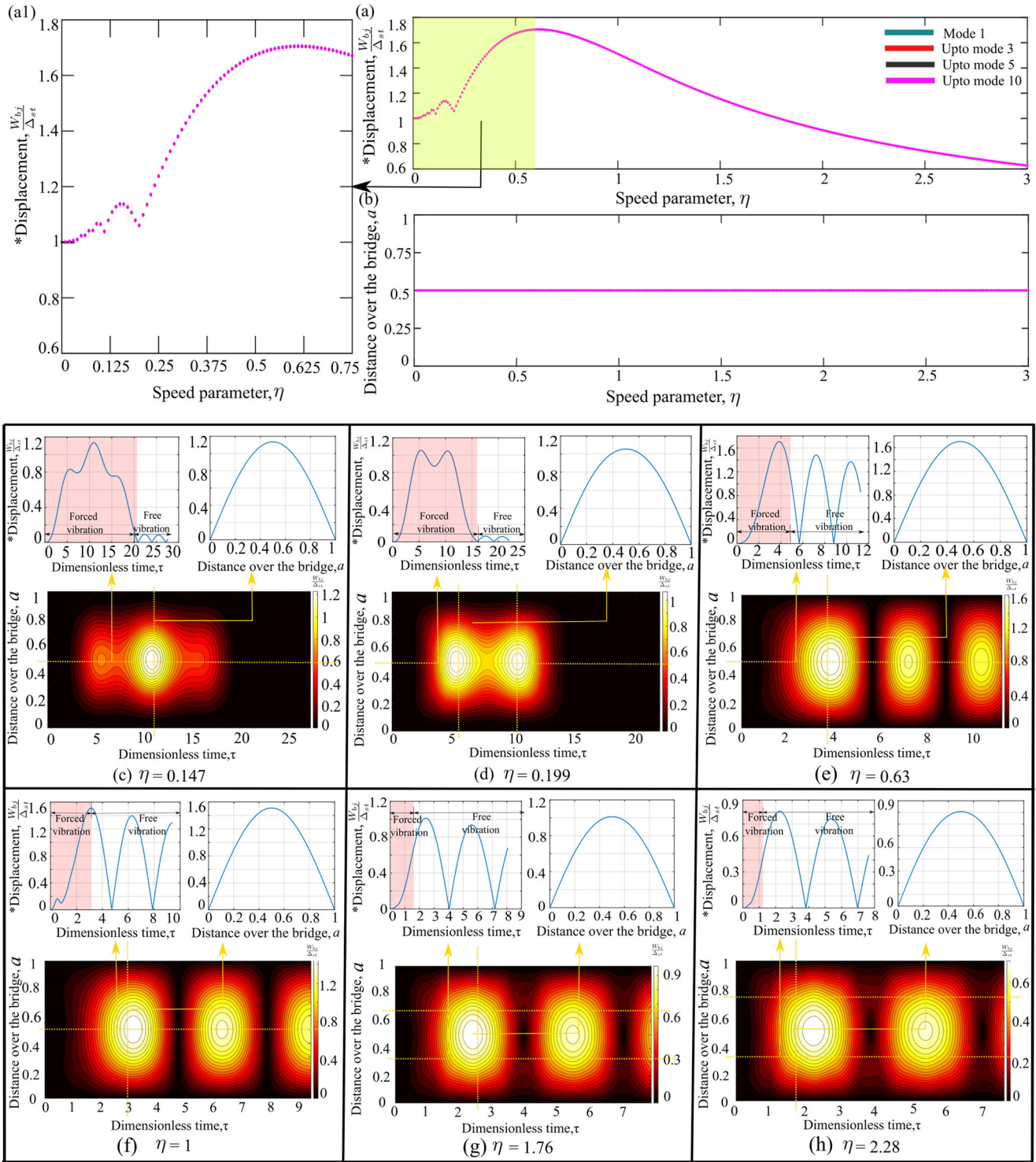
Figure 7. (a) *Dimensionless maximum displacement \frac{W_{bl}}{\Delta_{st}} ; (a1) enlarged view of Fig.(a) for \eta upto 0.7; (b) position a over the bridge ( a ) with respect to the speed parameter \eta ; (c) contour for \eta = 0.147 ; (d) contour for \eta = 0.199 ; (e) contour for \eta = 0.63 ; (f) contour for \eta = 1 ; (g) contour for \eta = 1.76 ; (h) contour for \eta = 2.28 with respect to time and length over the bridge a .
