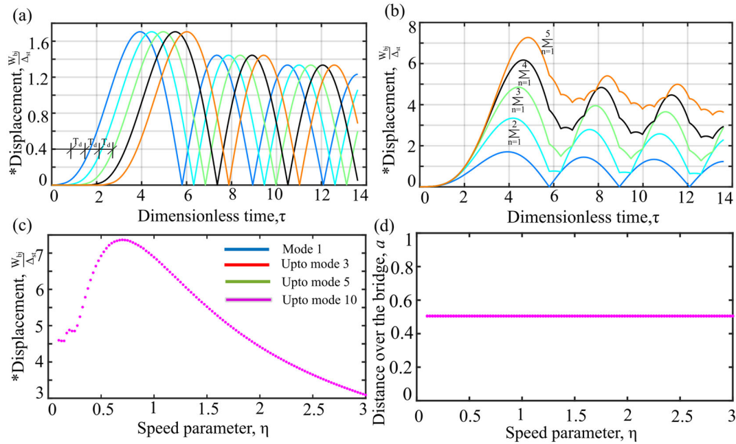
Figure 10. *Dimensionless displacement; (a) series of load ( N=5 ) with time lag \epsilon = 0.1 at \eta = 0.6 ; (b) Cumulative response of series of loads; (c) convergence of different modes; and (d) distance over the bridge a .
