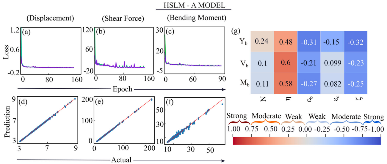
Figure 16. Loss versus epoch for (a) displacement; (b) shear force; (c) bending moment; Prediction versus actual for (d) displacement; (e) shear force; (f) Bending moment; and (g) Pearson correlation matrix for HSLM-A with the number of car units N -bogies, speed parameter \eta , the distance between loads to the length of the bridge \epsilon_b , the distance between consecutive car units to the length of the bridge \epsilon_c , and damping \zeta .
