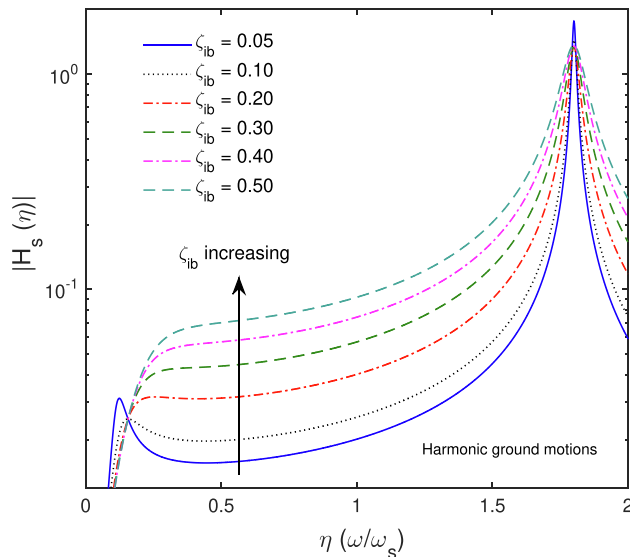
Fig. 6. Variations of displacement amplitudes of the structures isolated by IABI with frequency ratio for different value of \zeta_{ib} , subjected to harmonic base excitation.
