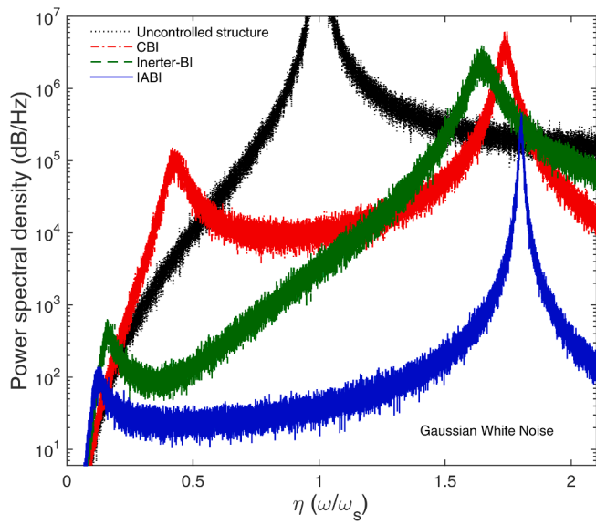
Fig. 5. Variations of power spectral density of the structures with frequency ratios.
