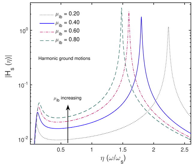
Fig. 7. Variations of displacement amplitudes of the structures isolated by IABI with frequency ratio for different value of \mu_{ib} , subjected to harmonic base excitation.
