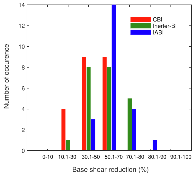
Fig. 13. Variation of number of occurrence with range of reduction percentage of the base shear.
