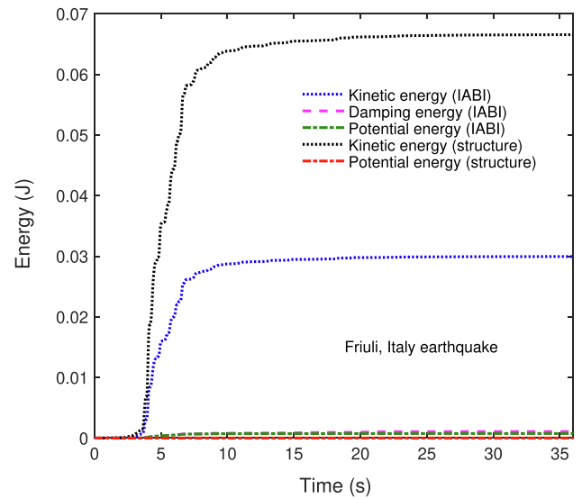
Fig. 16. (a) Energy plots of the structure isolated by inertial amplifier coupled base isolator under Friuli, Italy earthquake.
