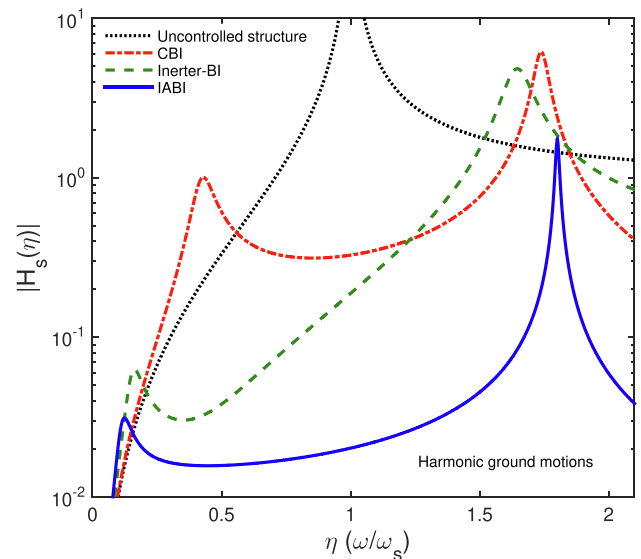
Fig. 4. (a) Variations of displacement amplitudes of structures with frequency ratios.
