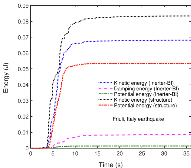
Fig. 15. (a) Energy plots of the structure isolated by inerter-based isolation system under Friuli, Italy earthquake.
