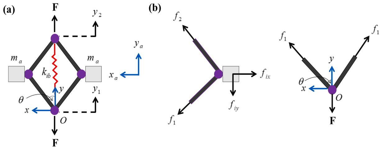
Fig. 2. (a) Schematic diagram of inertial amplifier (b) free-body diagram of inertial amplifier.
