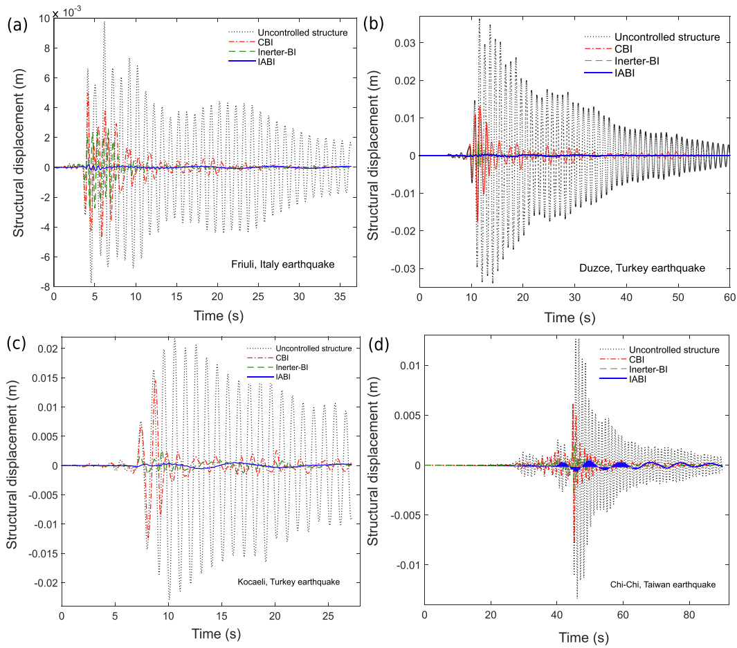
Fig. 10. Displacement history of the structures with time for different earthquake ground motion.
