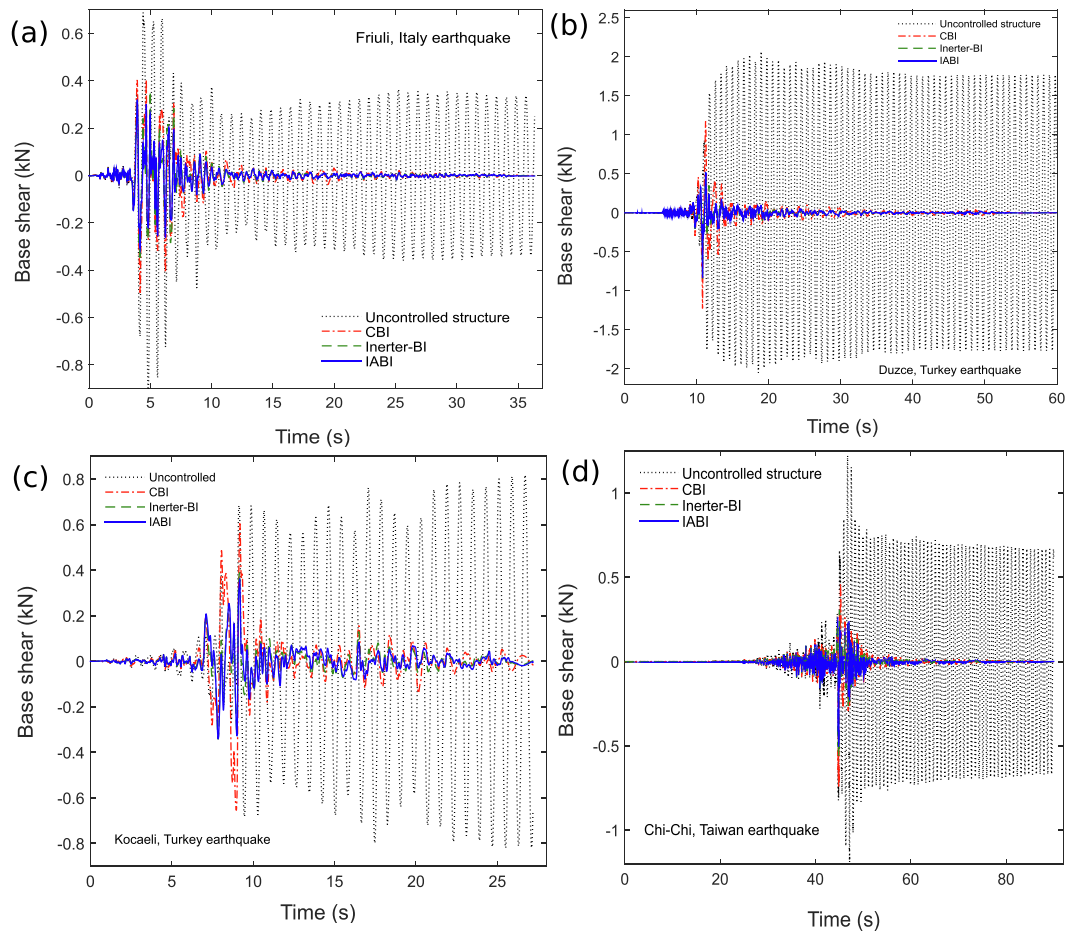
Fig. 12. (a–d) Variations of the base shear of the structure with time for different earthquakes.
