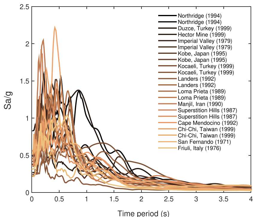
Fig. 9. Response spectra of the various earthquakes considered along with the designed spectra.
