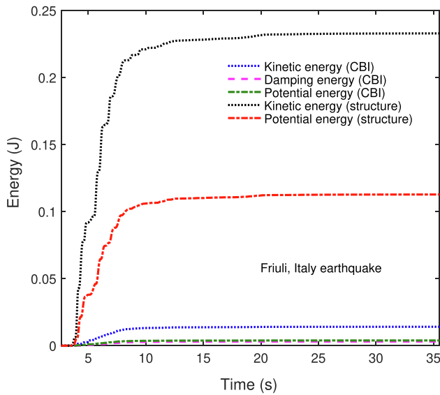
Fig. 14. (a) Energy plots of the structure isolated by classical base isolation system under Friuli, Italy earthquake.
