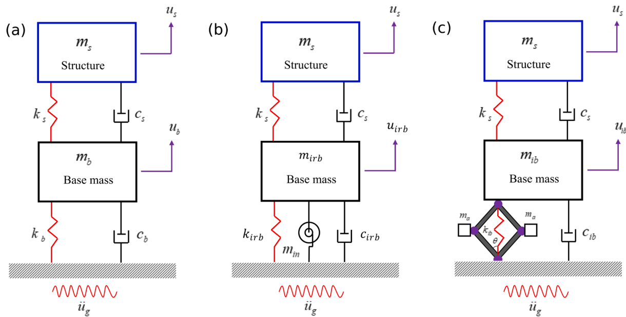
Fig. 1. Schematic diagrams of dynamic systems isolated by (a) classical base isolator, (b) inerter-based isolation system, (c) inertial amplifier coupled base isolator.
