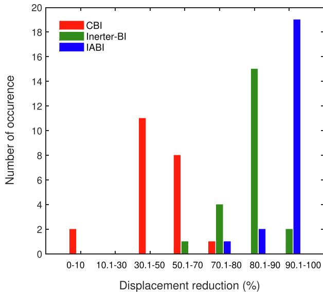
Fig. 11. Variation of number of occurrence with range of displacement reduction percentage.
