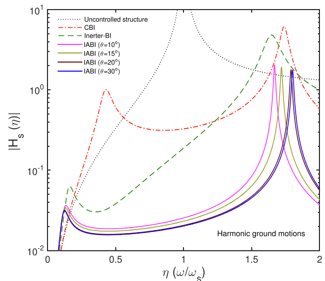
Fig. 8. Variations of displacement amplitudes of the structures isolated by IABI with frequency ratio for different value of \theta , subjected to harmonic base excitation.
