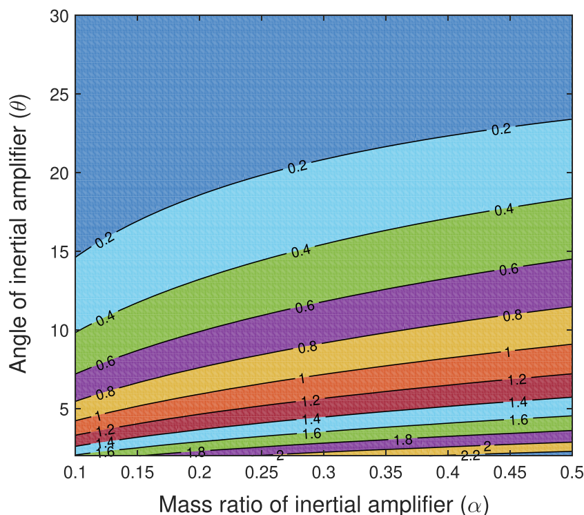
Fig. 3. Contours of \log_{10} of inertial amplification of IABI as a function of the inertial angle \theta and mass ratio \alpha .
