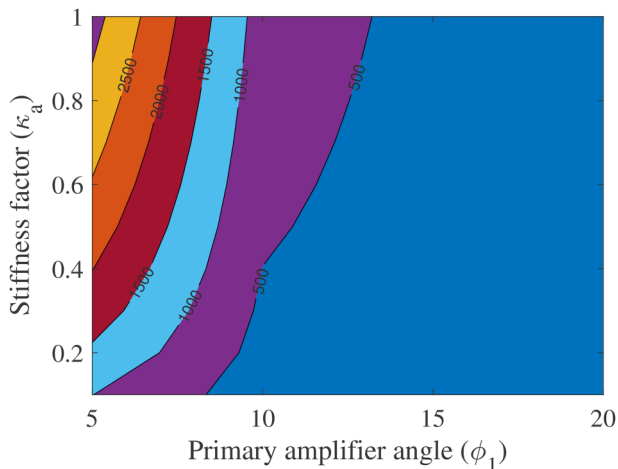
FIG. 7. The contour graph of Q-factor amplification coefficient as a function of the primary amplifier angle \phi_1 and stiffness factor \kappa_a for the cantilever with the compound stiffened inertial amplifier. The value of mass factor \mu_a is considered 0.1, and the secondary angle is considered \phi_2 = 70^\circ for this graph. The tertiary angle is considered \phi_3 = 15^\circ . For smaller amplifier angles \phi_1 \lesssim 10^\circ , the inertial amplification becomes prominent.
