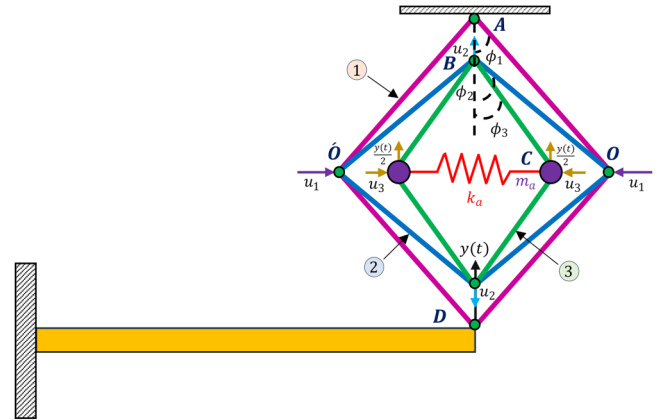
FIG. 4. A cantilever beam with the nested inertial amplifier. The nested inertial amplifier is made of three connected mechanisms. The mass m_a is placed inside the innermost mechanism. The amplifier angles for the mechanisms are \phi_1 , \phi_2 , and \phi_3 as shown. The displacement of the mass (at point D), points O, B, and C are denoted by y(t) , u_1(t) , u_2(t) , and u_3(t) , respectively. The forces F_i(t) , i = 1, \dots, 4 are the internal forces within the rigid links of the mechanism 1, 2, and 3, respectively.
