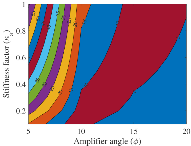
FIG. 6. The contour graph of the Q-factor amplification coefficient as a function of the amplifier angle \phi and stiffness factor \kappa_a for the cantilever with the compound stiffened inertial amplifier. The value of mass factor \mu_a is considered 0.1, and the secondary angle is considered \theta = 70^\circ for this graph. For smaller amplifier angles \phi \lesssim 10^\circ , the inertial amplification becomes prominent.
