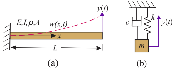
FIG. 1. Schematic diagrams of (a) A damped cantilever beam, and (b) The equivalent damped single degree of freedom (SDOF) oscillator model.
