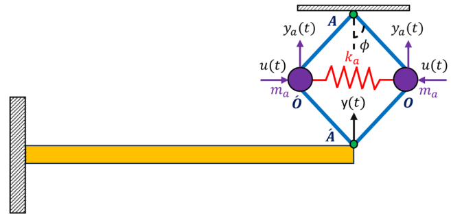
FIG. 2. A small amplitude free vibration is applied to a cantilever beam that is equipped with a stiffened inertial amplifier. The amplifier is affixed to the upper portion of the cantilever beam. The static mass, rigidity, and damping of the beam are expressed as m , k , and c , correspondingly. Two masses m_a are located at the two horizontal terminals of the inertial amplifier. The amplifier's rigidity, k_a , is determined by the spring that connects these two masses. The amplifier angle, denoted as \phi , is the angle formed by the rhombus-type structural configuration of the inertial amplifier at its joints. y(t) and u(t) represent the displacement of the amplifier (at point O) and the apex of the beam (at point A). The static mass, stiffness, and damping of the cantilever beam are increased to the effective mass, stiffness, and damping, which are m_e , k_e , and c , as a result of these deflections. The Q-factor of the cantilever beam is improved by its effective attenuation.
