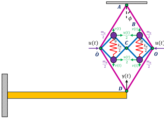
FIG. 3. A cantilever beam with compound inertial amplifier. A compound inertial amplifier with two cells. The primary amplifier angle is \phi , and the secondary amplifier angle is \theta . Each mass within the cells is m_a/2 so that the total mass is the same as the conventional inertial amplifier. The displacement of the mass (at point D), point O, and the amplifier mass (at point B) are denoted by y(t) , u(t) , and v(t) , respectively. The forces F_1(t) , F_2(t) , and F_3(t) are the internal forces within the rigid links of the primary and secondary mechanisms.
