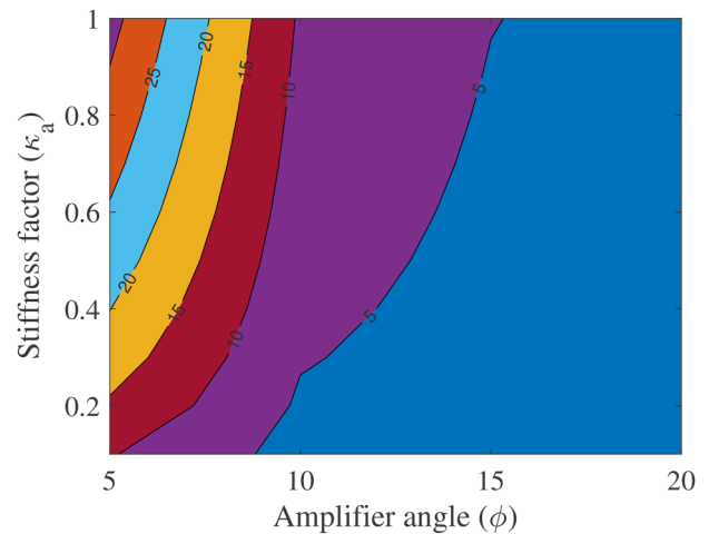
FIG. 5. The contour graph of the Q-factor amplification coefficient as a function of the amplifier angle \phi and stiffness factor \kappa_a for the cantilever with the stiffened inertial amplifier. The value of mass factor \mu_a is considered 0.1 for this graph. For smaller amplifier angles \phi \lesssim 10^\circ , the inertial amplification becomes prominent.
