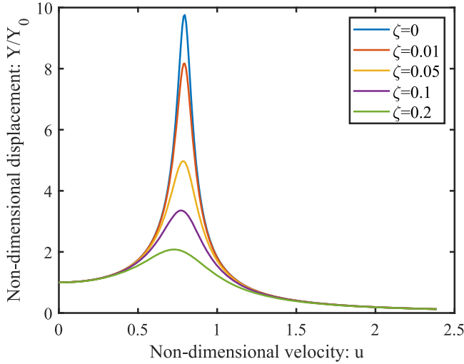
Figure 5. The non-dimensional displacement amplitude of a harvester with an inductor as a function of the non-dimensional free stream velocity for five selected values of damping factors.
