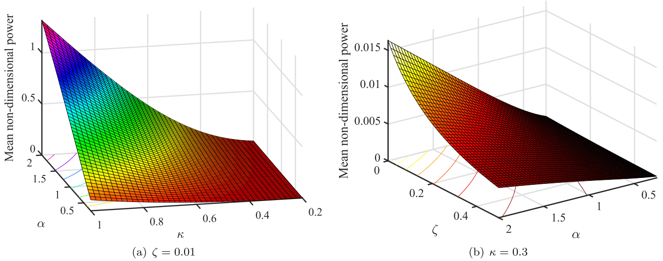
Figure 9. The mean of non-dimensional harvested power from the vortex induced vibration as functions of \alpha , \zeta and \kappa . The normalised random field parameters are \hat{\sigma} = 1 and \hat{\nu} = 1 .
