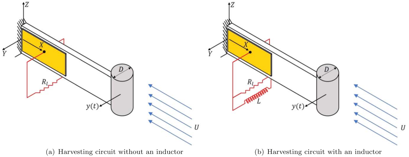
Figure 2. Schematic diagrams of vortex-induced piezoelectric vibration energy harvesters with two different harvesting circuits.
