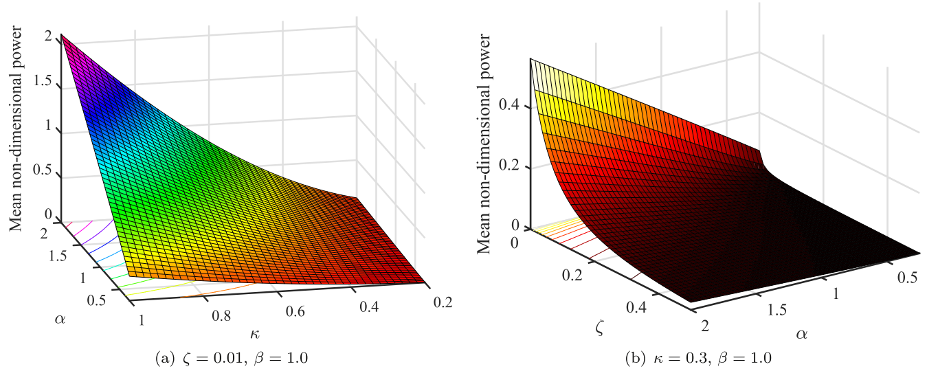
Figure 10. The mean of non-dimensional harvested power from the vortex induced vibration as functions of \alpha , \zeta and \kappa . The value of the inductor constant is fixed at \beta = 1.0 . The normalised random field parameters are \hat{\sigma} = 1 and \hat{\nu} = 1 .
