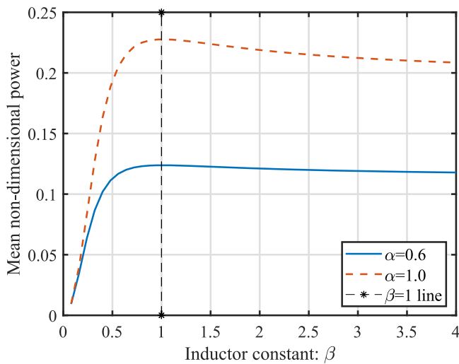
Figure 12. The mean of non-dimensional harvested power for a harvester with an inductor as a function of \beta for two values of \alpha with fixed values of \zeta = 0.01 and \kappa = 0.3 . The * corresponds to the optimal value of \beta (=1) for the maximum mean harvested power.
