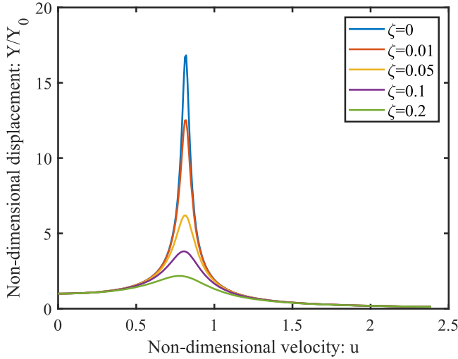
Figure 3. The non-dimensional displacement amplitude of a harvester without an inductor as a function of the non-dimensional free stream velocity for five selected values of damping factors.
