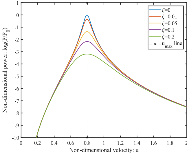
Figure 6. The non-dimensional power of a harvester with an inductor as a function of the non-dimensional free stream velocity for five selected values of damping factors.
