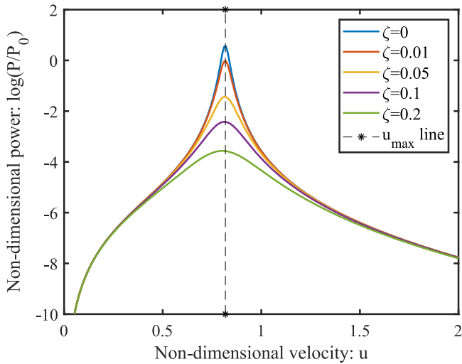
Figure 4. The non-dimensional power of a harvester without an inductor as a function of the non-dimensional free stream velocity for five selected values of damping factors.
