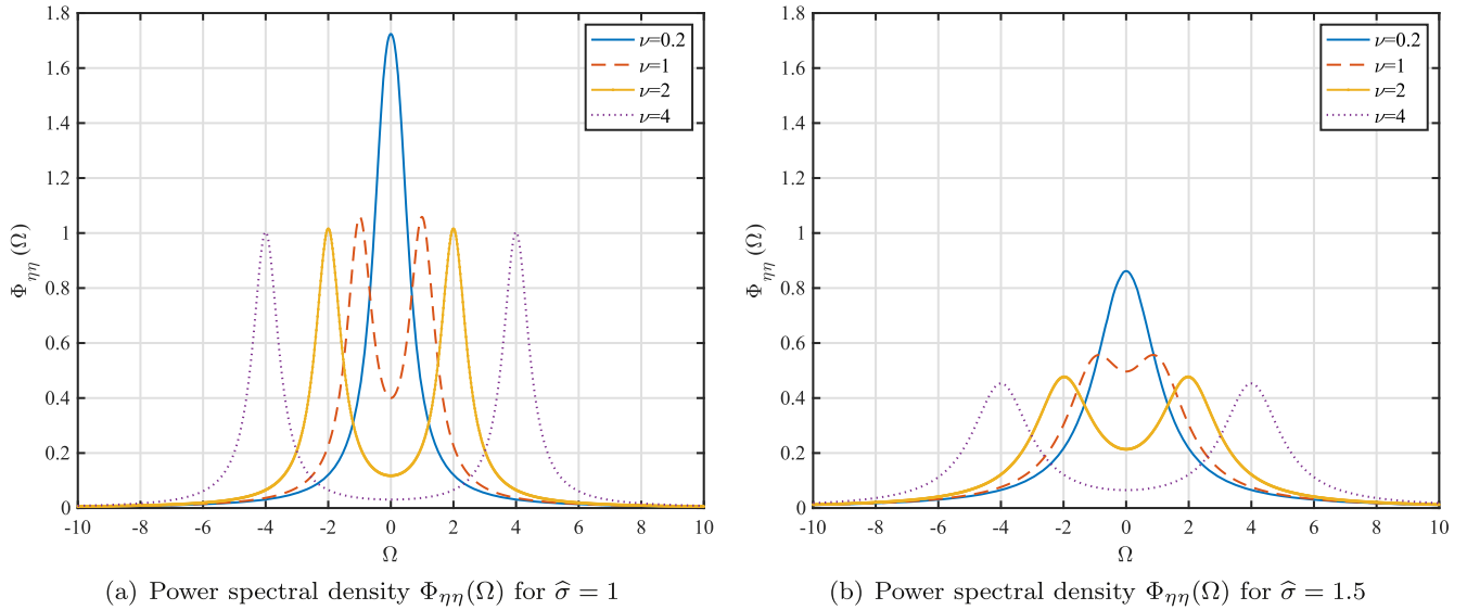
Figure 8. The power spectral density the forcing random process \eta(t) for four different values of non-dimensional central frequency \hat{\nu} .
