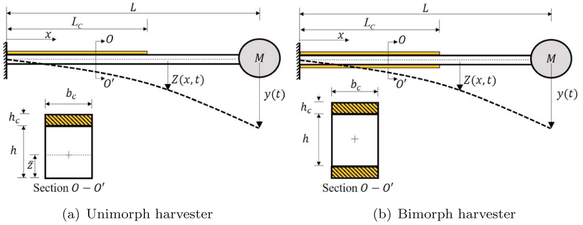
Figure 1. Cantilever vibration energy harvesters with unimorph and bimorph configurations. The length of the cantilever is L and the mass of the bluff body attached at the tip is M .
