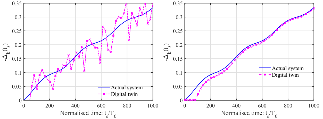
(a) Digital twin constructed with erroneous data (b) Digital twin constructed with error estimate
