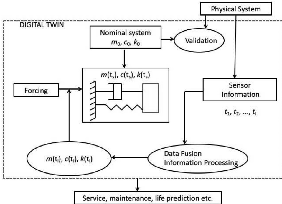
Fig. 1. The overview of constructing a digital twin for a single-degree-of-freedom dynamic system.
