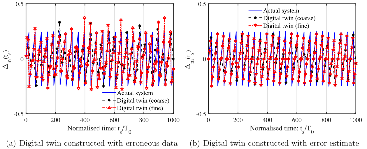
Fig. 6. Digital twin constructed with erroneous data and error estimates as a function of the normalised ‘slow time’ t_s/T_0 . Error in the form of a discrete zero-mean Gaussian white noise with a standard deviation of 0.025 is considered.
