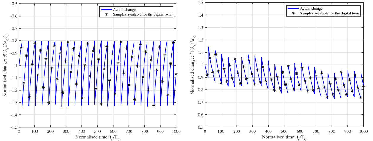
(a) Changes in the real part of the natural frequency (b) Changes in the imaginary part of the natural frequency
