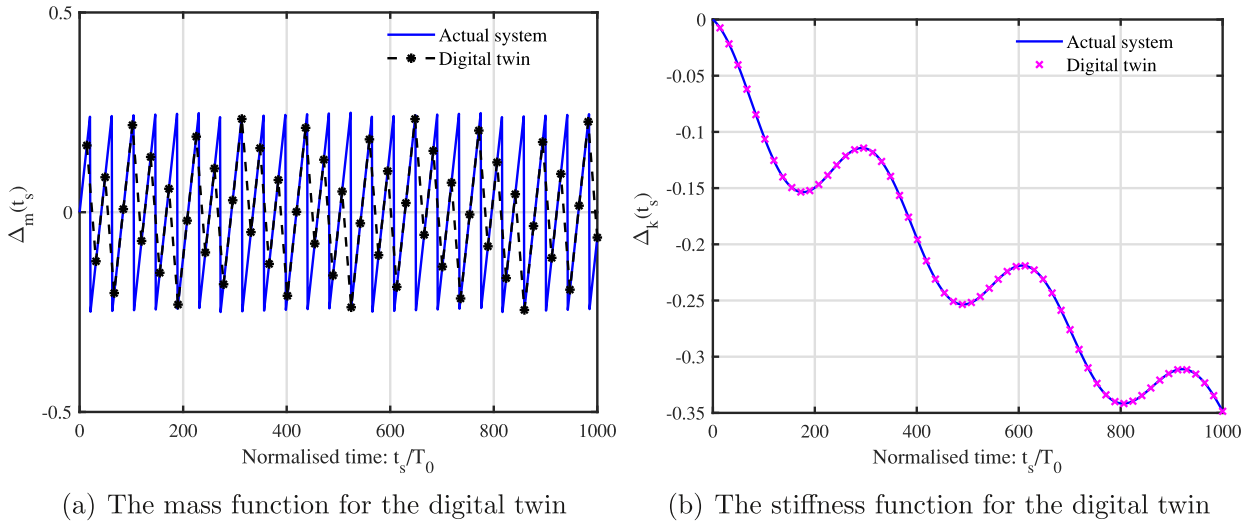
Fig. 8. Digital twin obtained from coarse but exact data via simultaneous mass and stiffness evolution as a function of the normalised ‘slow time’ t_s/T_0 . The mass function in (a) is obtained using (58) while the stiffness function in (b) is obtained using (59).
