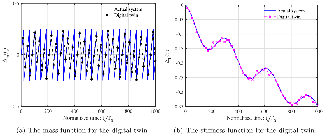
Fig. 10. Digital twin obtained with error estimates via simultaneous mass and stiffness evolution as a function of the normalised ‘slow time’ t_s/T_0 . The mass function in (a) is obtained using (69) while the stiffness function in (b) is obtained using (70). Errors in the form of a discrete zero-mean Gaussian white noise with standard deviations of 0.025 and 0.025\zeta_0 are considered for the imaginary and real parts.
