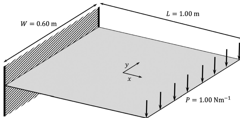
Fig. 12. Plate system.
