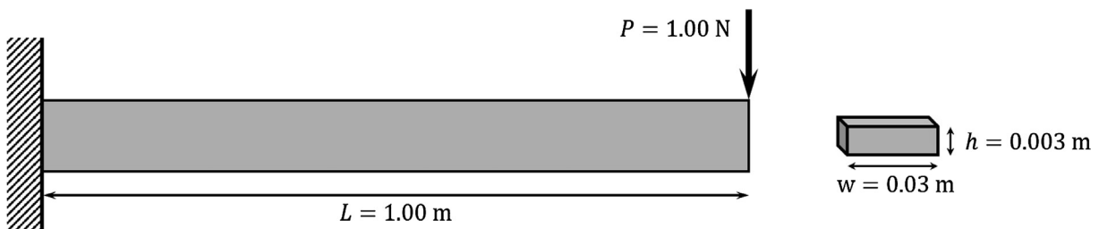
Fig. 1. Beam system.
