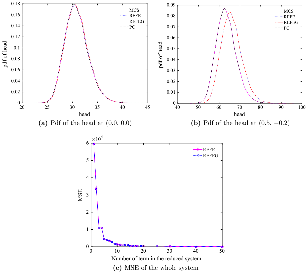
Fig. 11. Pdfs of the head (cm) at (0.0, 0.0) and (0.5, -0.2) and the mean square error of the whole system when using REFE and REFEG for different truncation values of Eqs. (17) and (38).
