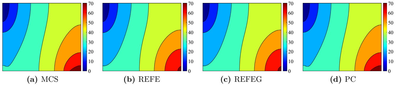
Fig. 8. Contour plots of the mean of the head (cm) obtained with the MCS, REFE, REFEG and PC methods. The x and y axis are respectively the positions in the x direction with x \in [-0.5, 0.5] m and in the y direction with y \in [-0.3, 0.3] m.
