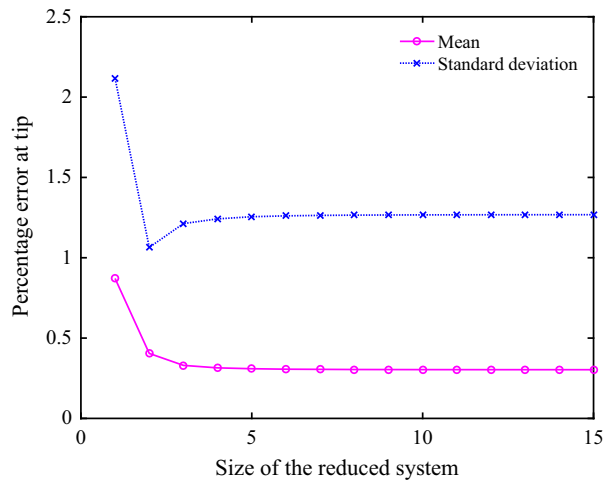
(b) Error of mean and standard deviation - REFE
