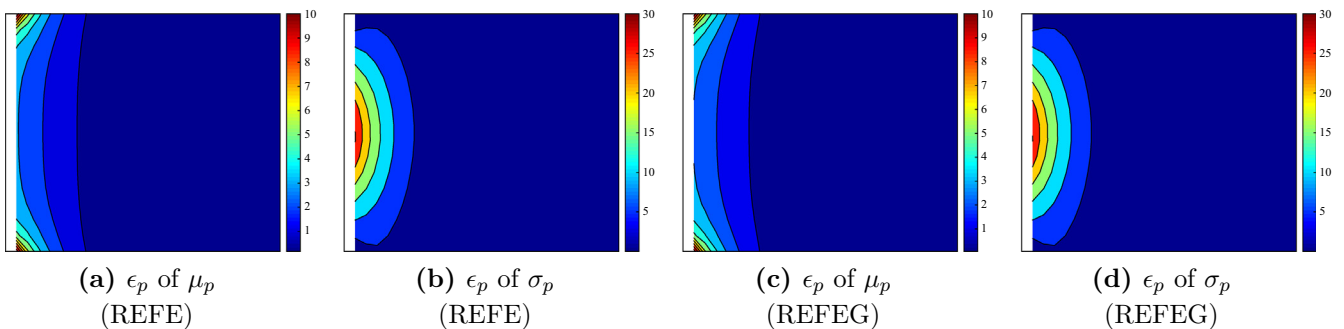
Fig. 16. Contour plots of the percentage error ( \epsilon_p ) of the mean and standard deviation of the REFE and REFEG methods compared to the MCS method. The x and y axis are respectively the positions in the x direction with x \in [-0.5, 0.5] \text{ m} and in the y direction with y \in [-0.3, 0.3] \text{ m} .
