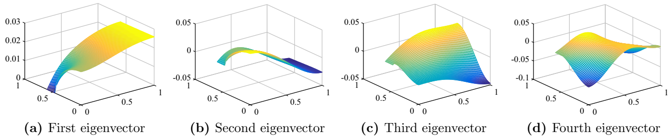
Fig. 7. First four eigenvectors of the stiffness matrix for the flow through porous media problem.
