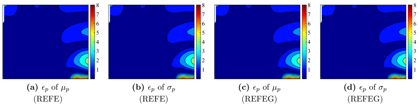
Fig. 10. Contour plots of the percentage error ( \epsilon_p ) of the mean ( \mu_p ) and standard deviation ( \sigma_p ) of the REFE and REFEG methods compared to the MCS method. The x and y axis are respectively the positions in the x direction with x \in [-0.5, 0.5] m and in the y direction with y \in [-0.3, 0.3] m.
