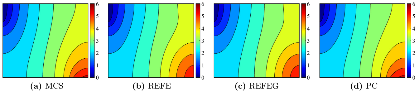
Fig. 9. Contour plots of the standard deviation of the head (cm) obtained with the MCS, REFE, REFEG and PC methods. The x and y axis are respectively the positions in the x direction with x \in [-0.5, 0.5] m and in the y direction with y \in [-0.3, 0.3] m.
