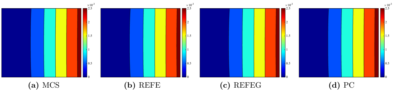
Fig. 15. Contour plots of the standard deviation of the vertical displacement (m) of the plate when applying the MCS, REFE, REFEG and PC methods. The x and y axis are respectively the positions in the x direction with x \in [-0.5, 0.5] \text{ m} and in the y direction with y \in [-0.3, 0.3] \text{ m} .
