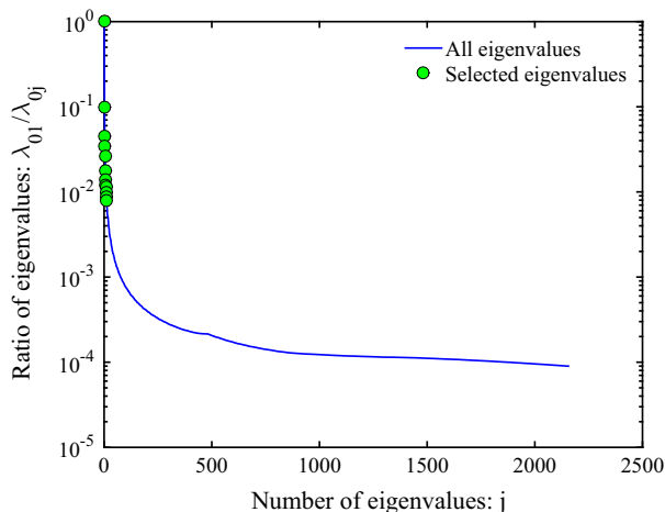
Fig. 6. Ratio of eigenvalues for the flow through porous media problem.
