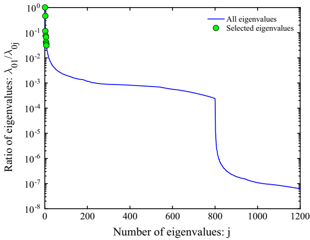
Fig. 13. Ratio of eigenvalues for the bending of an elastic plate problem.
