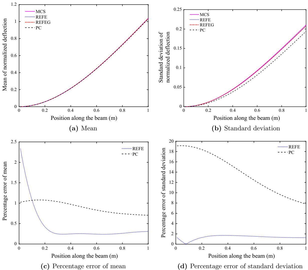
Fig. 3. The mean and the standard deviation of the normalised vertical displacement of the beam and a comparison of the percentage error of the mean and the standard deviation of the normalised vertical displacement between the MCS and REF methods.
