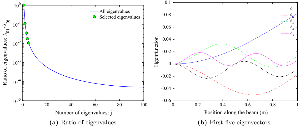
Fig. 2. Ratio of eigenvalues and the first five eigenvectors of the beam problem.
