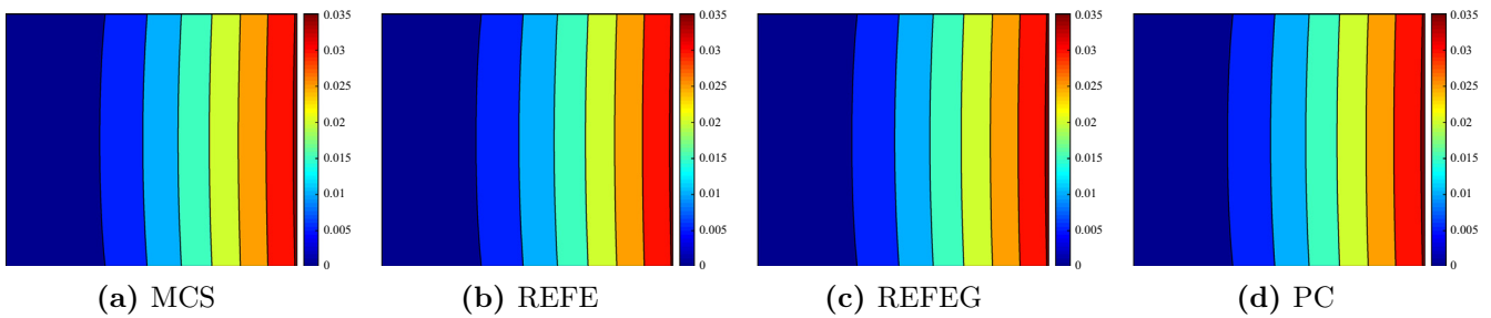
Fig. 14. Contour plots of the mean of the vertical displacement (m) of the plate when applying the MCS, REFE, REFEG and PC methods. The x and y axis are respectively the positions in the x direction with x \in [-0.5, 0.5] \text{ m} and in the y direction with y \in [-0.3, 0.3] \text{ m} .
