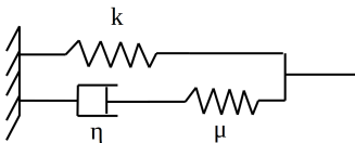
(i) Standard linear model
