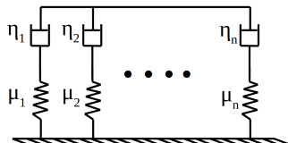
(j) Generalised Maxwell model
