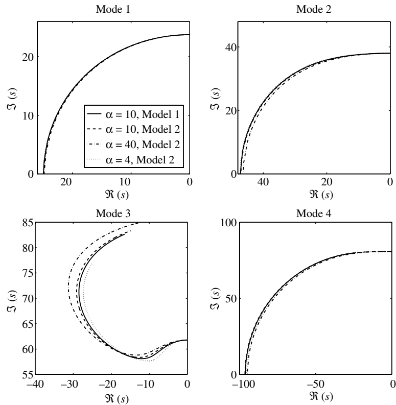
Fig. 15. The root loci of first four eigenvalues of the simply supported rectangular plate with external damping as H_0 increases from 0 to 8 \times 10^3 (for \mu = \infty ).
