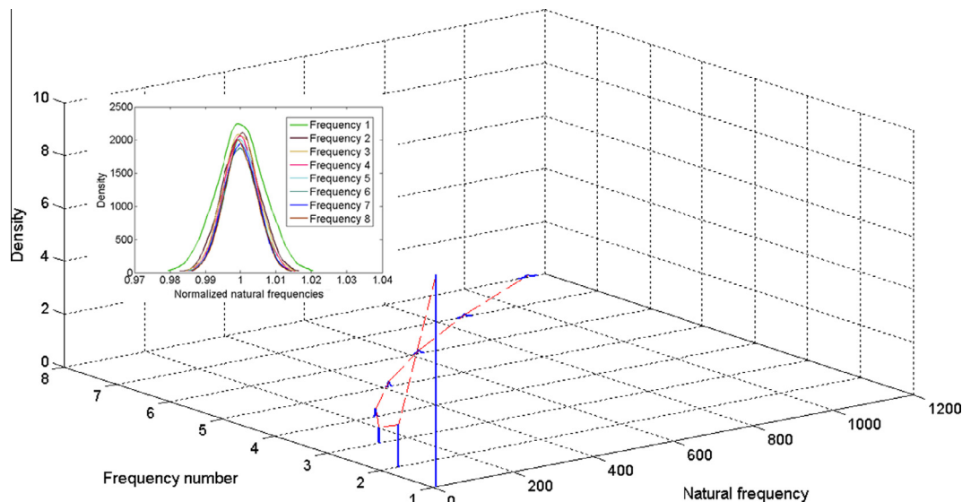
Fig. 25. Probability density function plots for the first eight natural frequencies corresponding to bending modes. In the inset, normalized natural frequencies with respect to their respective mean values are shown.
