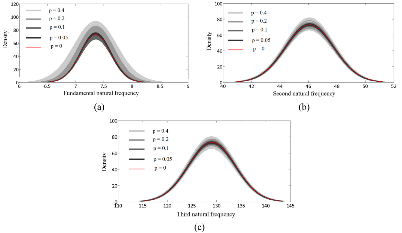
Fig. 27. Probability density function plots depicting the effect of noise on RBF based uncertainty quantification for first three natural frequencies.
