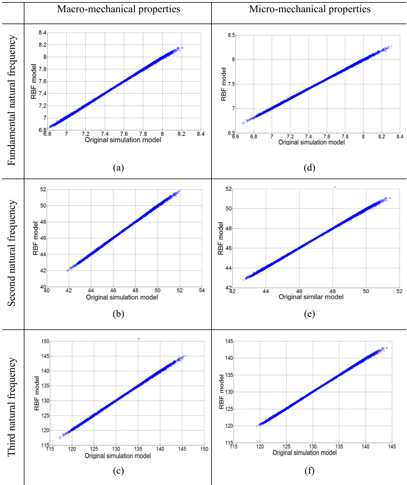
Fig. 10. (a–c) Scatter plot of macro-mechanical properties obtained by original MCS and RBF model with respect to first three natural frequencies for circular thin walled composite beam, considering sample size = 10,000, with \theta = 30^\circ , m = 16 , n = 18 ; (d–f) Scatter plot of micro-mechanical properties obtained by original MCS and RBF model with respect to first three natural frequencies for circular thin walled composite beam, considering sample size = 10,000, with \theta = 30^\circ , m = 16 , n = 18 .
