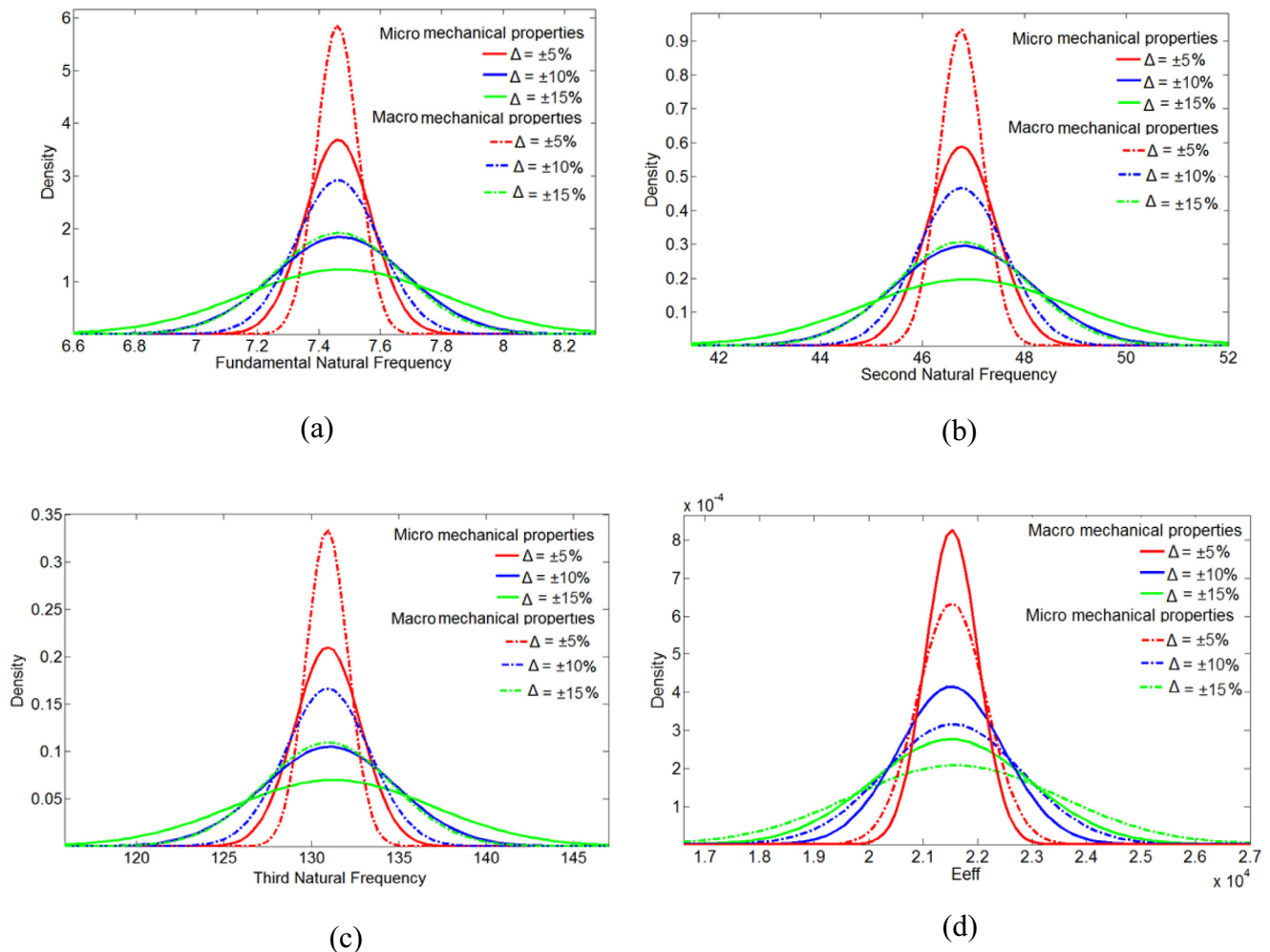
Fig. 17. (a–c) Probability density function plots for first three natural frequencies considering different degree of stochasticity ( \Delta ); (d) Probability density function plot for the effective longitudinal modulus considering different degree of stochasticity ( \Delta ).
