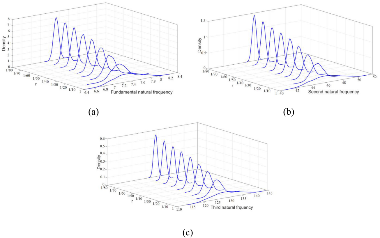
Fig. 21. Probability density function plots for first three natural frequencies considering spatially random variation of micro-material properties.
