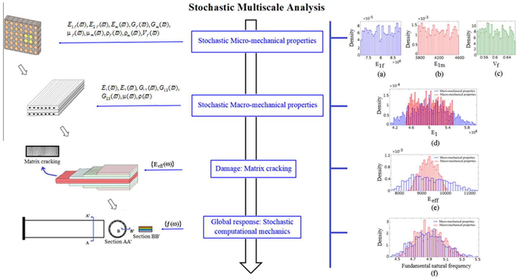
Fig. 12. Proposed stochastic multiscale analysis scheme of laminate composite beam with matrix cracking (In figures, d–f the histograms in blue and red colour indicate micro-mechanical and macro-mechanical properties respectively). (For interpretation of the references to colour in this figure legend, the reader is referred to the web version of this article.)
