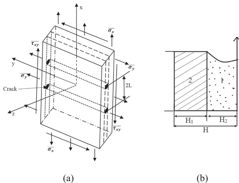
Fig. 2. (a) Laminated composite containing cracked ply; (b) One-quarter of laminated composite unit-cell.
