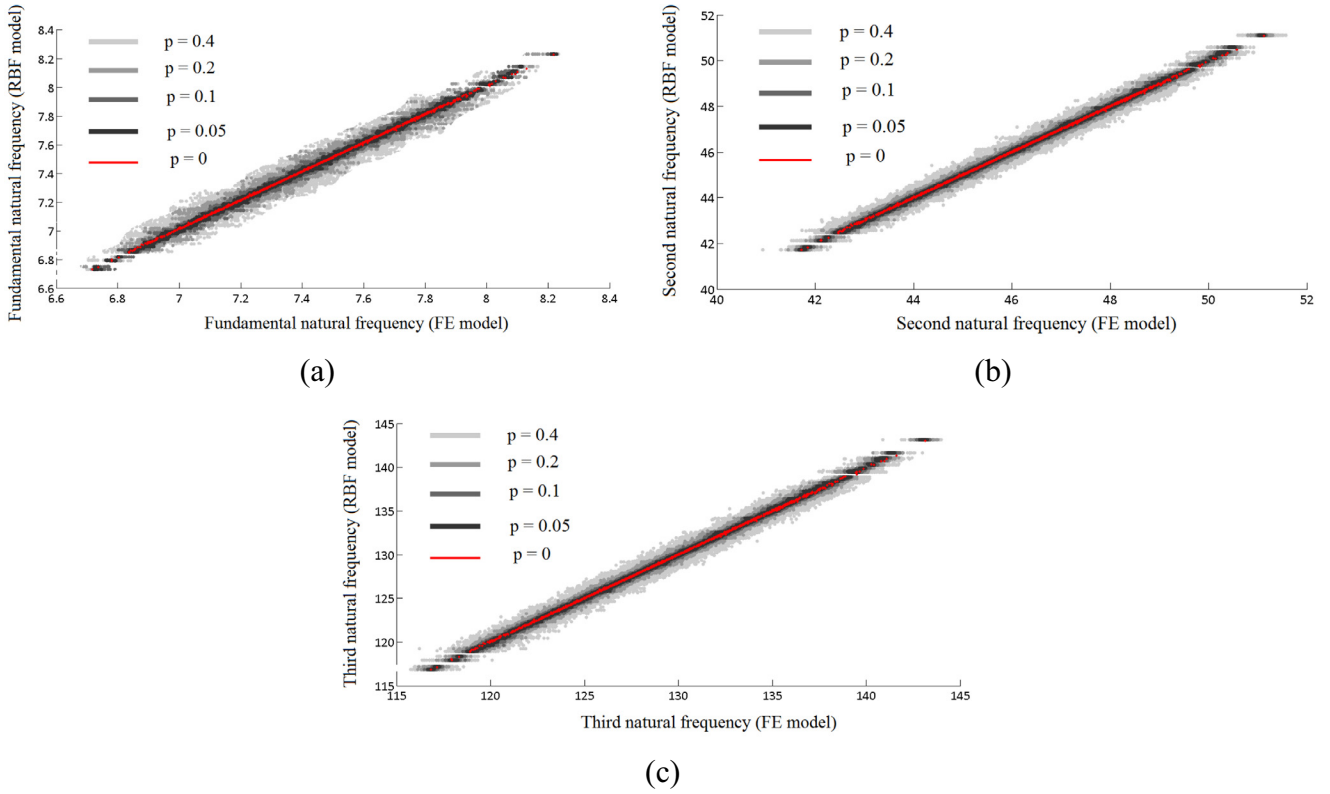
Fig. 26. Scatter plots depicting the effect of noise on RBF based uncertainty quantification for first three natural frequencies.
