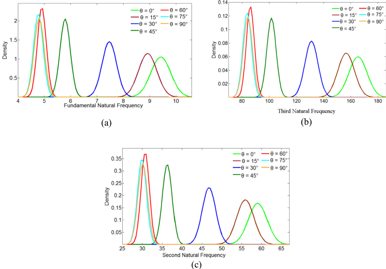
Fig. 13. (a–c) Probability density function plots for first three natural frequencies for different fibre orientation angle ( \theta ).
