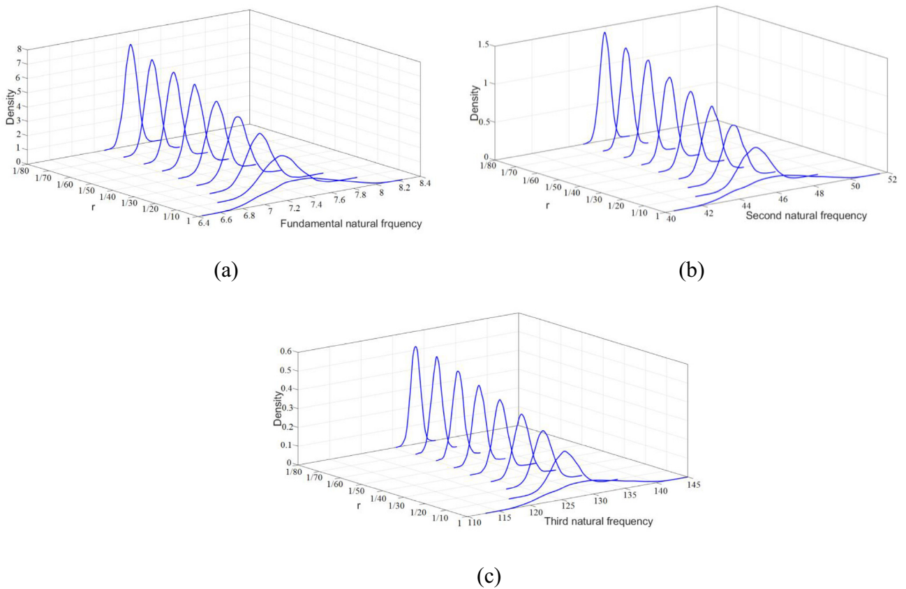
Fig. 23. Probability density function plots for first three natural frequencies considering combined spatially random variation of micro-material properties and crack densities.
