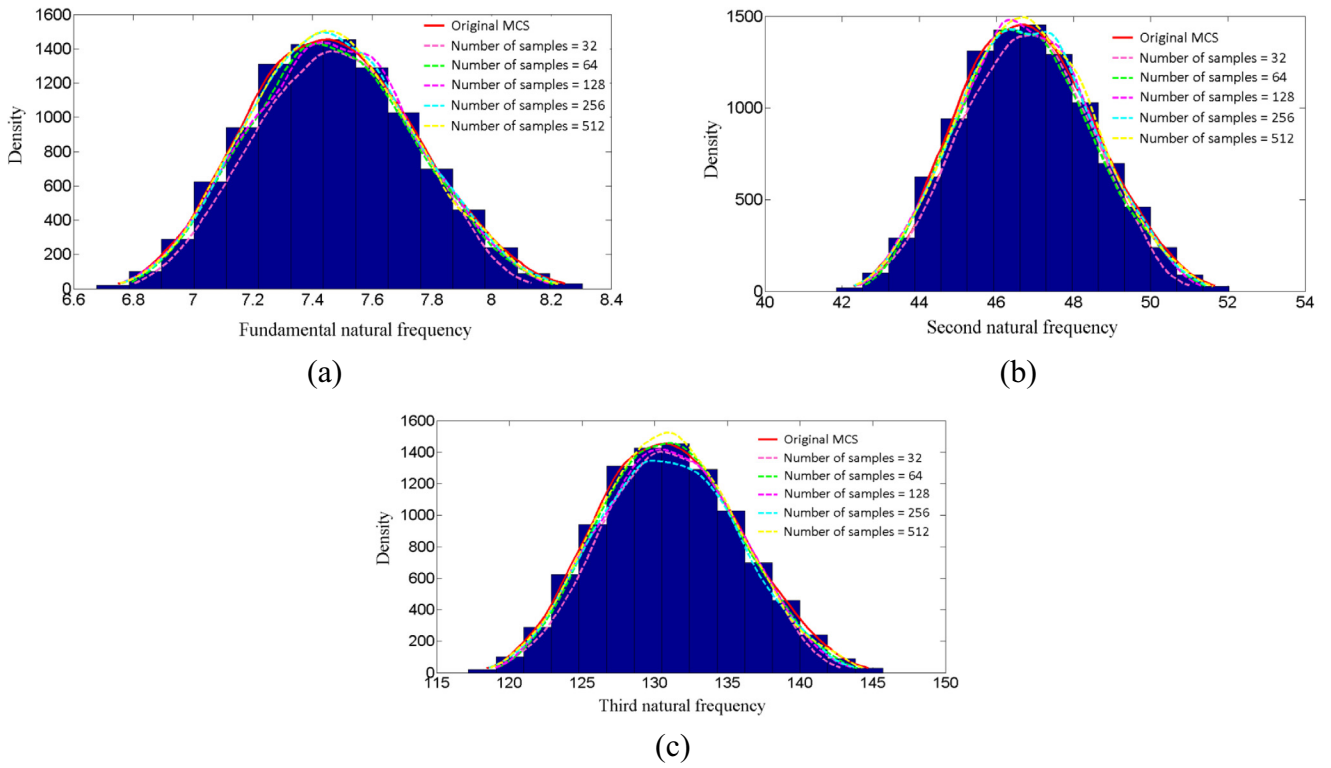
Fig. 8. Probability density function plots for different sample sizes of Sobol sampling considering stochasticity in micro-mechanical properties along with original MCS.
