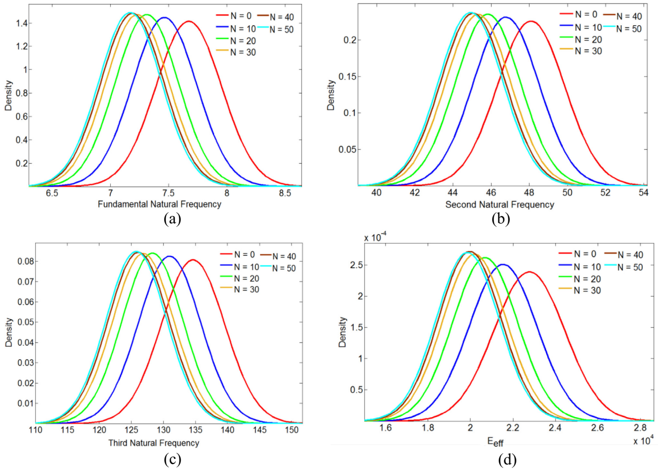
Fig. 18. (a–c) Probability density function plot for first three natural frequencies, considering different crack densities ( N ), with fibre orientation angle \theta = 30^\circ , m = 16 , n = 18 , degree of stochasticity ( \Delta ) = \pm 10\% in micro-mechanical properties (d) Probability density function plot for effective longitudinal modulus ( E_{eff} ) considering different crack densities, with fibre orientation angle \theta = 30^\circ , m = 16 , n = 18 and degree of stochasticity ( \Delta ) = \pm 10\% in micro-mechanical properties.
