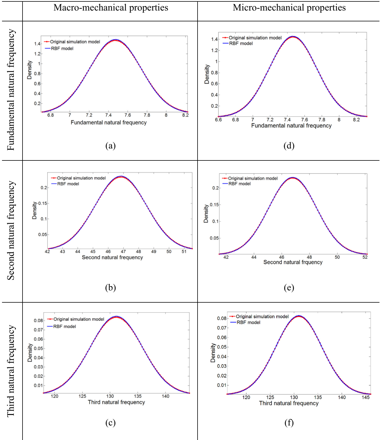
Fig. 11. (a–c) Probability density function of macro-mechanical properties obtained by original MCS and RBF model with respect to first three natural frequencies for circular thin walled composite beam, considering sample size = 10,000, with \theta = 30^\circ , m = 16 , n = 18 ; (d–f) Probability density function of micro-mechanical properties obtained by original MCS and RBF model with respect to first three natural frequencies for circular thin walled composite beam, considering sample size = 10,000, with \theta = 30^\circ , m = 16 , n = 18 .
