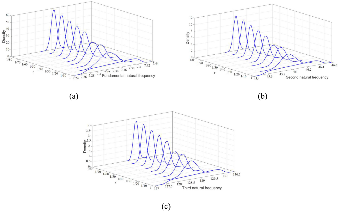
Fig. 22. Probability density function plots for first three natural frequencies considering spatially random variation of crack densities.
