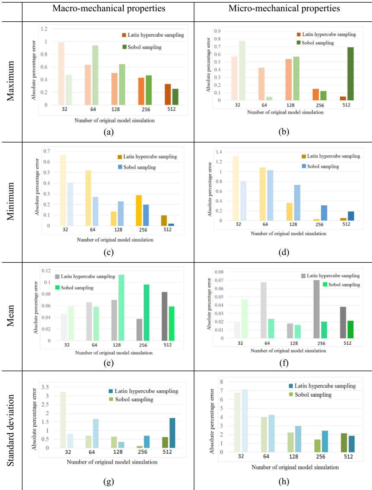
Fig. 7. Absolute percentage error in maximum, minimum, mean and standard deviation of fundamental natural frequencies with respect to original MCS for micro and macro mechanical properties obtained for different sample sizes considering LHS and Sobol sampling.
