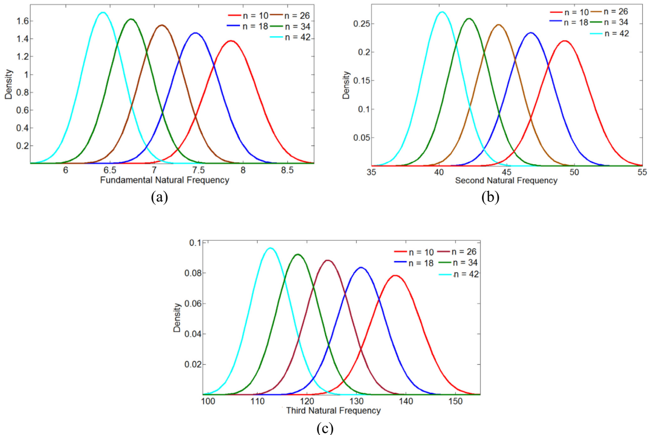
Fig. 14. (a–c) Probability density function plots for first three natural frequencies corresponding to various numbers of ply numbers having ply orientation angle of 90° (n).
