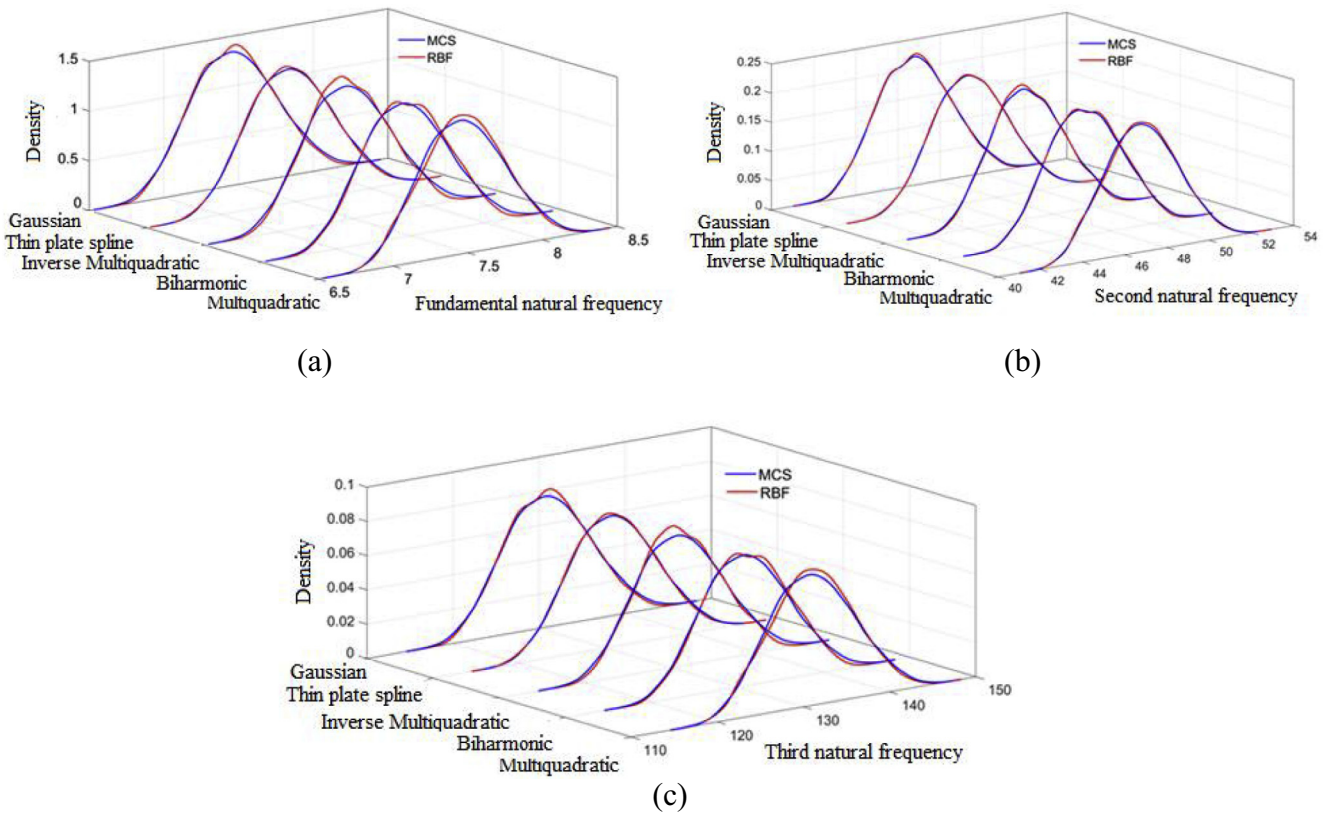
Fig. 9. Performance of different basis functions for constructing RBF model corresponding to first three natural frequencies.
