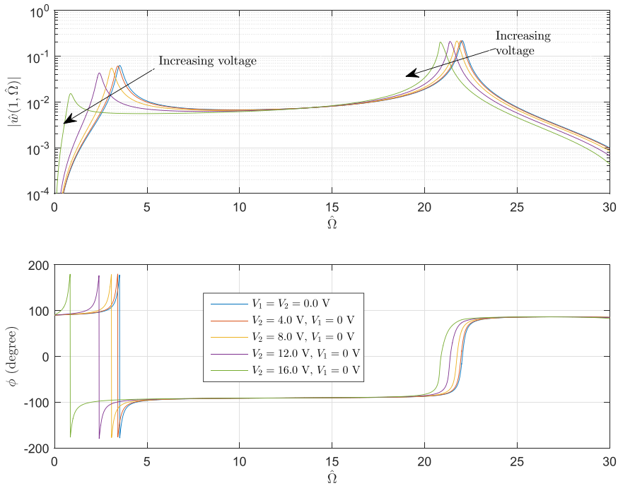
Fig. 11. Frequency and phase responses of the beam-tip displacement (case 3).
