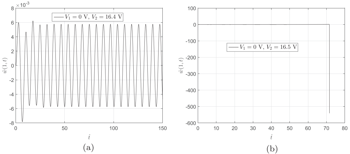
Fig. 10. Non-dimensionalized tip displacement time histories at \hat{\Omega} = 0.873 and (a) V_1 = 0 \text{ V}, V_2 = 16.4 \text{ V} and (b) V_1 = 0 \text{ V}, V_2 = 16.5 \text{ V} .
