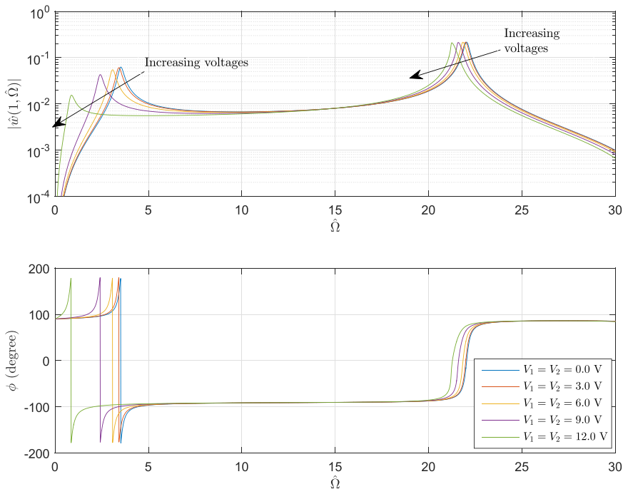
Fig. 5. Frequency and phase responses of the beam-tip displacement (case 1).
