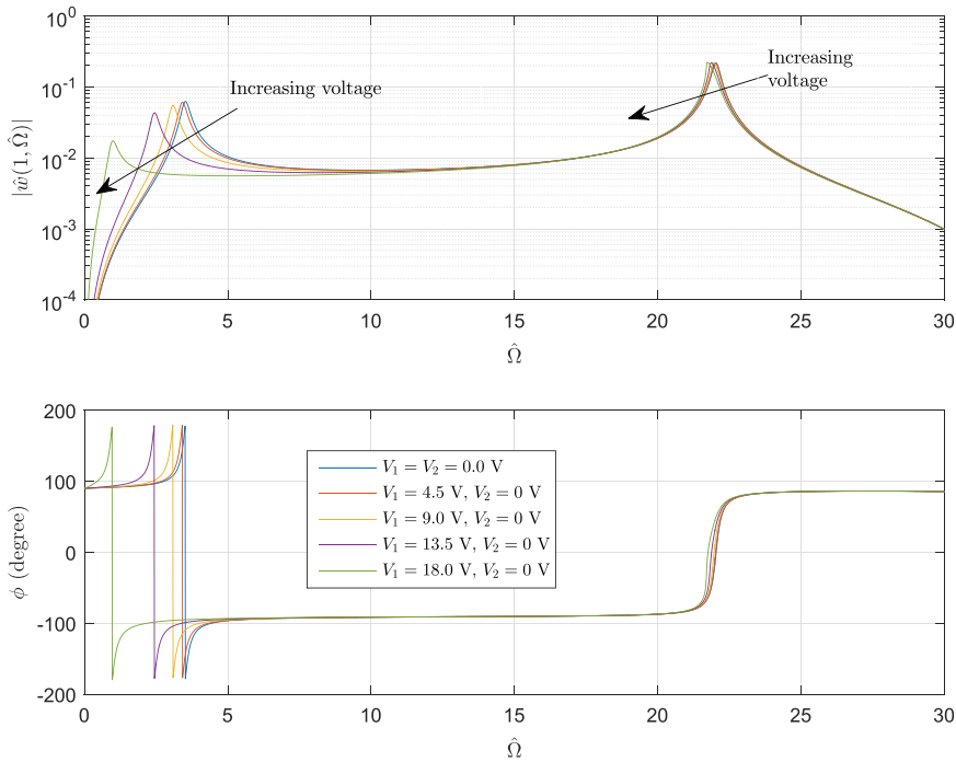
Fig. 8. Frequency and phase responses of the beam-tip displacement (case 2).
