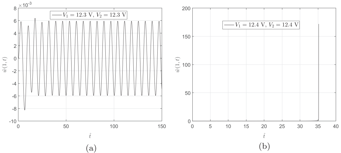
Fig. 4. Non-dimensionalized tip displacement time histories at \hat{\Omega} = 0.873 and (a) V_1 = V_2 = 12.3 V and (b) V_1 = V_2 = 12.4 V.
