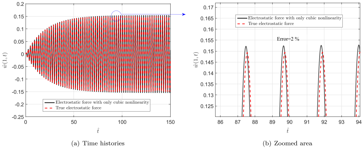
Fig. 2. Non-dimensionalized tip displacement time histories for the system with only cubic non-linearity (solid line) and the system with true electrostatic force (dashed line), V_1 = V_2 = 7 \text{ V} , z_0 = 0.1 \mu\text{m} , \hat{\Omega} = 2.891 , (a) Time histories (b) Zoomed area.
