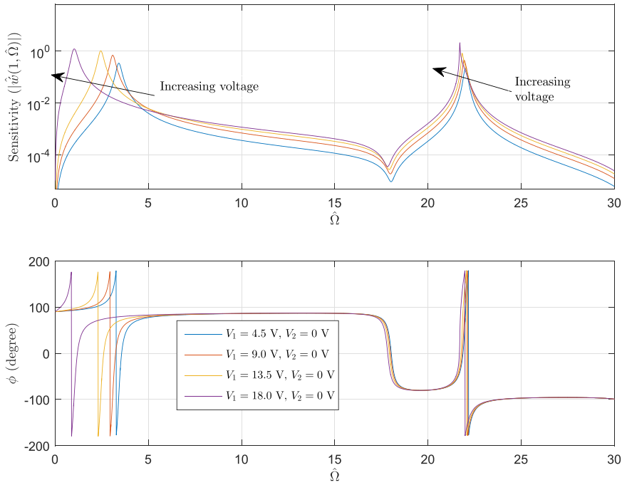
Fig. 9. Sensitivity of frequency and phase responses of the beam-tip displacement with respect to V_1 (case 2).
