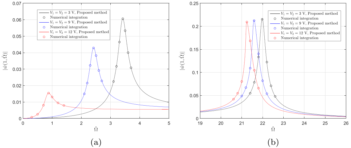
Fig. 3. Validation of the results (a) mode 1 and (b) mode 2.
