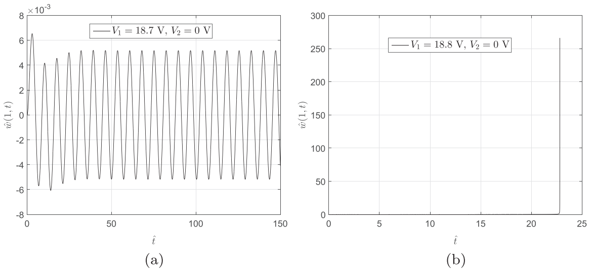
Fig. 7. Non-dimensionalized tip displacement time histories at \hat{\Omega} = 0.873 and (a) V_1=18.7 \text{ V}, V_2 = 0 \text{ V} and (b) V_1=18.8 \text{ V}, V_2 = 0 \text{ V} .
