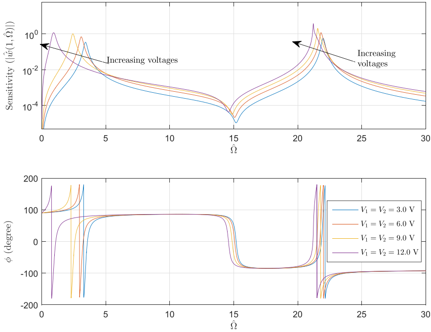
Fig. 6. Sum of sensitivities of frequency and phase responses of the beam-tip displacement with respect to V_1 and V_2 (case 1).
