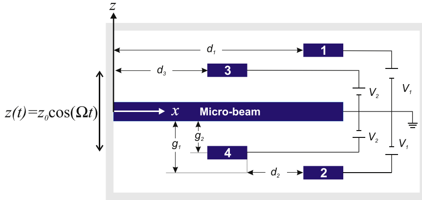
Fig. 1. Schematic of the MEMS device.
