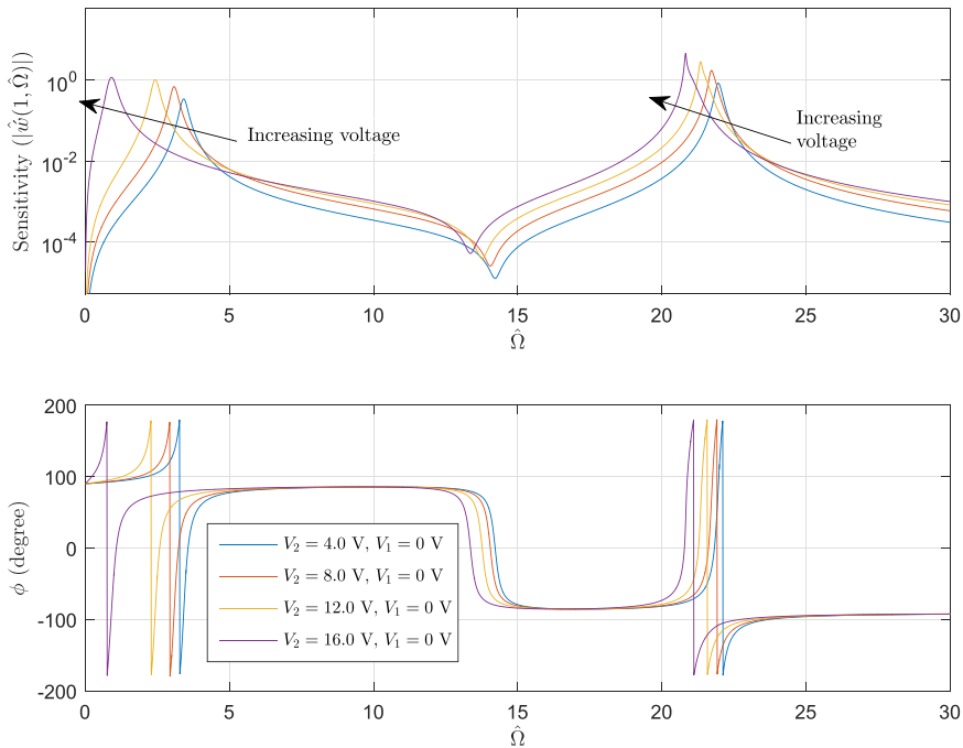
Fig. 12. Sensitivity of frequency and phase responses of the beam-tip displacement with respect to V_2 (case 3).
